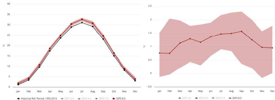
Figure 17-7 Projected Climatology (Left) and Anomaly (Right) of Average Mean Surface Air Temperature for 2020-2039 (Annual) for the Project Region; (Ref. Period: 1995-2014), SSP5-8.5, Multi-Model Ensemble
