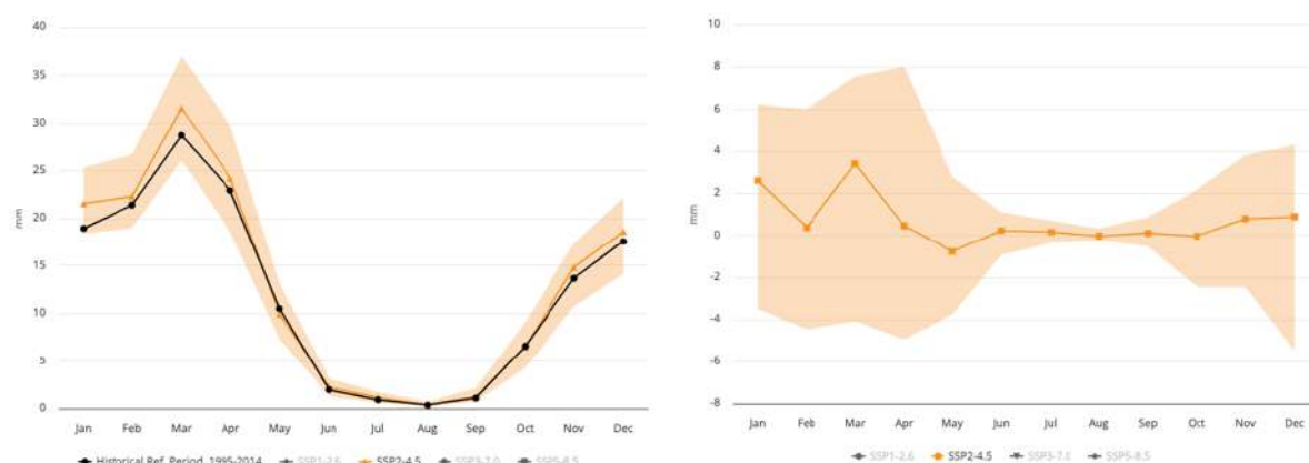
Figure 17-20 Projected Precipitation Climatology (Left) and Anomaly (Right) for 2020-2039 (Annual) for the Project Region; (Ref.Period: 1995-2014), SSP2-4.5, Multi-Model Ensemble
