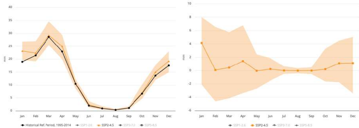
Figure 17-21 Projected Precipitation Climatology (Left) and Anomaly (Right) for 2040-2059 (Annual) for the Project Region; (Ref.Period: 1995-2014), SSP2-4.5, Multi-Model Ensemble
