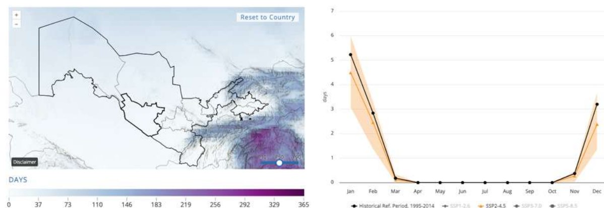
Figure 17-15 Projected Number of Ice Days (Tmax < 0°C) for the Project Area (2020-2039), SSP2-4.5, 50 th Percentile
