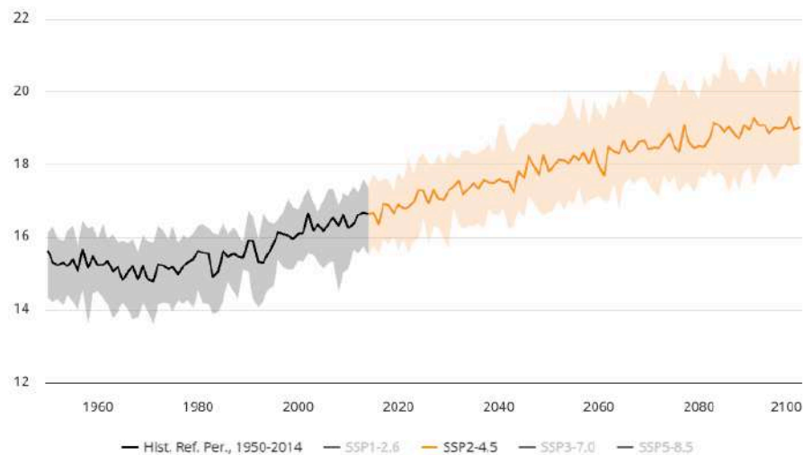
Figure 17-6 Projected Average Mean Surface Air Temperature for the Project Region; (Ref. Period: 1995-2014), SSP2-4.5, Multi-Model Ensemble
