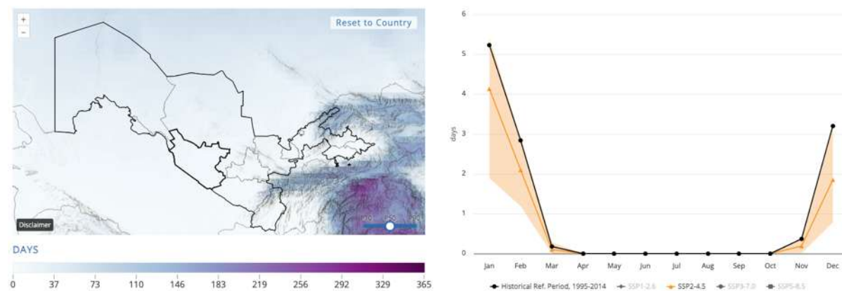
Figure 17-16 Projected Number of Ice Days (Tmax < 0°C) for the Project Area (2040-2059), SSP2-4.5, 50 th Percentile
