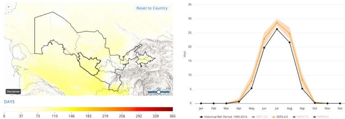
Figure 17-10 Projected Number of Hot Days ( T_{max} > 35^{\circ}\text{C} ) for the Project Area (2020-2039), SSP2-4.5, 50 th Percentile
