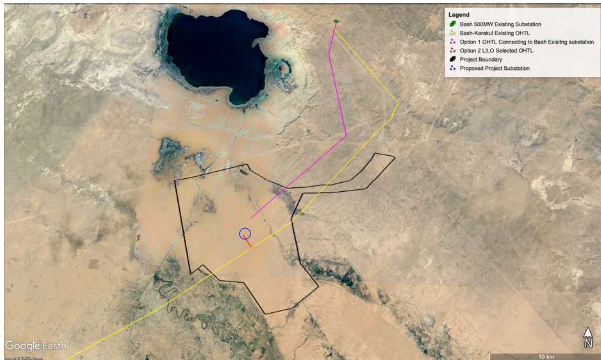
Figure 2-21 OHTL Options Considered and the Selected Route show in Red
