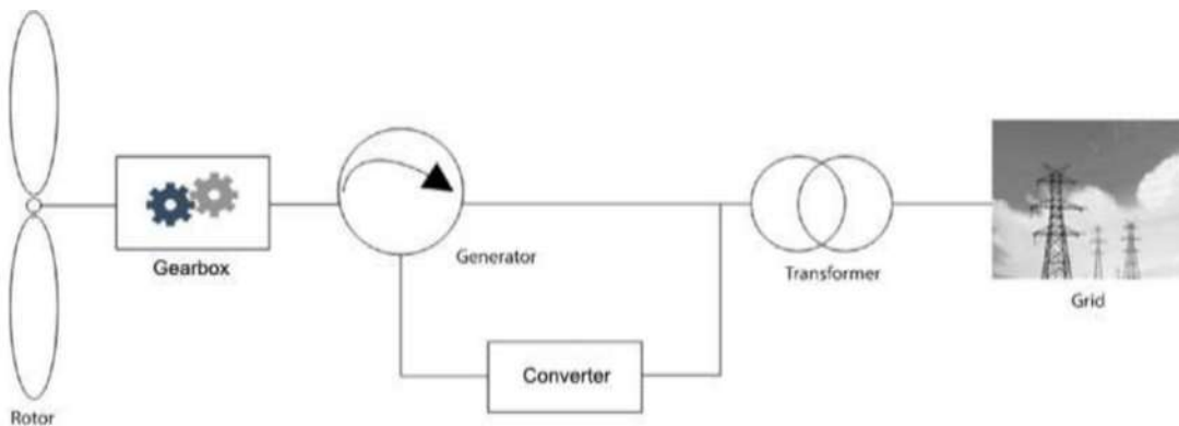
Figure 2-12 Schematic of the Electrical System – Electrical Drive Chain for DFAG
