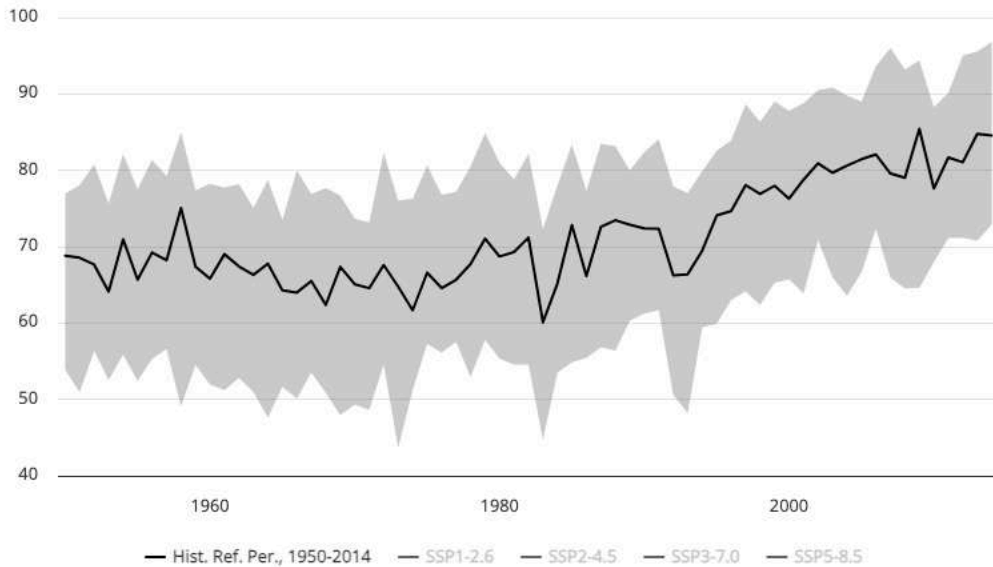
Figure 17-2 Historical Climatology of Number of Hot Days (Tmax > 35°C) per Year for 1950-2014 in the Project Area, Multi-Model Ensemble
