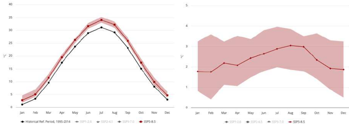
Figure 17-8 Projected Climatology (Left) and Anomaly (Right) of Average Mean Surface Air Temperature for 2040-2059 (Annual) for the Project Region; (Ref. Period: 1995-2014), SSP5-8.5, Multi-Model Ensemble
