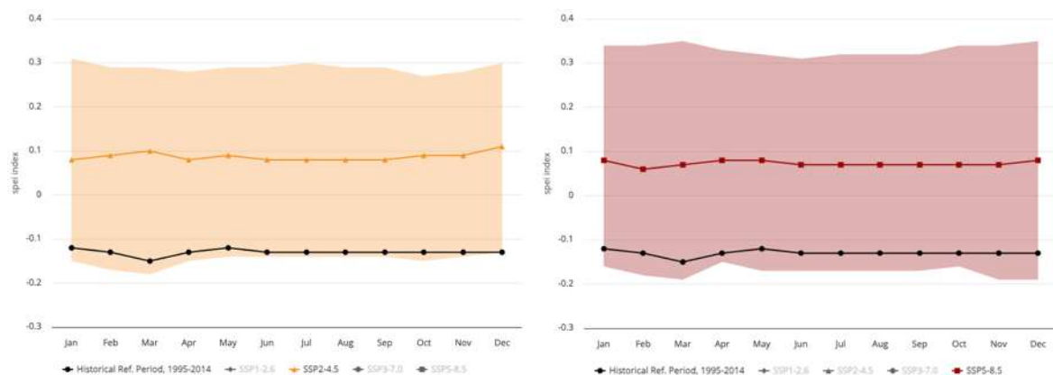
Figure 17-29 Projected Climatology of Annual SPEI Drought Index for 2040-2059 (Annual) for the Project Region; (Ref. Period: 1995-2014), SSP2-4.5 (Left) SSP5-8.5 (Right), Multi-Model Ensemble
