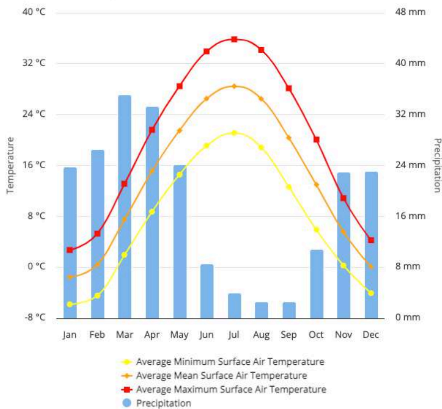
Figure 17-1 1 Average Monthly Climate Conditions in the Project Area for 1991-2022 (CCKP, 2024)
