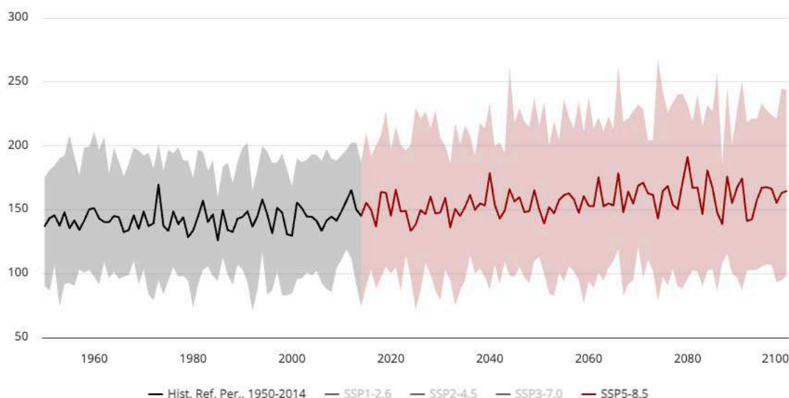
Figure 17-25 Projected Precipitation in the Project Region; (Ref. Period: 1995-2014), SSP5-8.5, Multi-Model Ensemble
