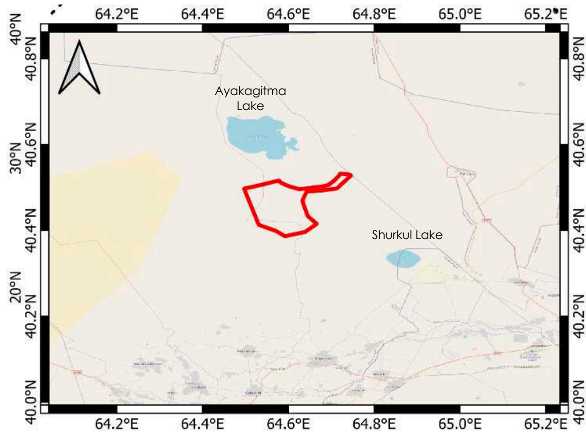
Figure 8-3 Lakes in the Project Area (UzAssystem, 2024c) 17
