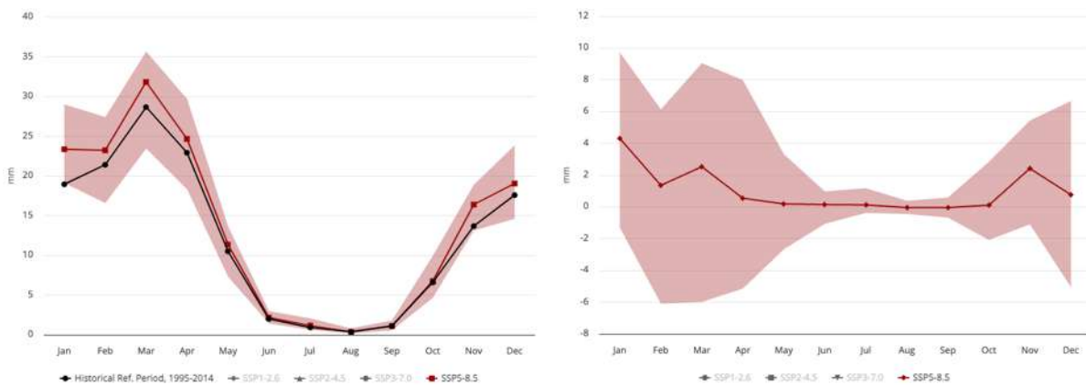
Figure 17-24 Projected Precipitation Climatology (Left) and Anomaly (Right) for 2040-2049 (Annual) for the Project Region; (Ref. Period: 1995-2014), SSP5-8.5, Multi-Model Ensemble
