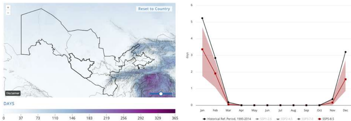
Figure 17-18 Projected Number of Ice Days ( T_{max} < 0^{\circ}\text{C} ) for the Project Area (2040-2059), SSP5-8.5, 50 th Percentile
