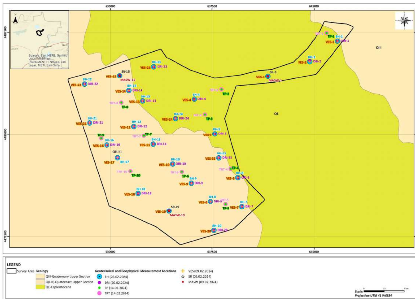
Figure 8-1 Geological Map of the Project Site (UzAssystem, 2024a)
