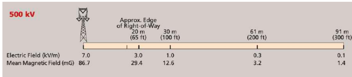
Figure 15-1 Typical EMF levels for Power Transmission Lines
