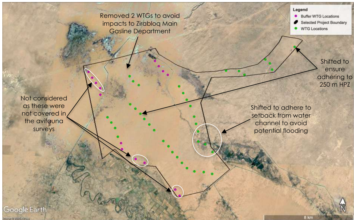
Figure 2-19 July 2024 WTG Distribution
