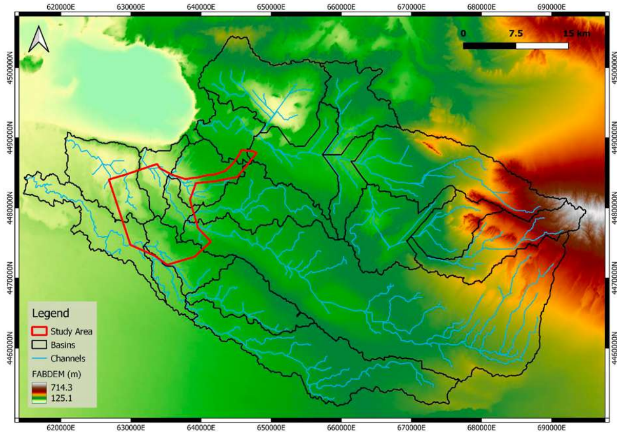
Figure 8-5 Watershed in the Project Area (UzAssystem, 2024c) 17
