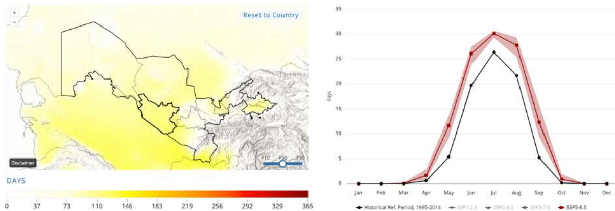
Figure 17-13 Projected Number of Hot Days ( T_{max} > 35^{\circ}\text{C} ) for the Project Area (2040-2059), SSP5-8.5, 50 th Percentile
