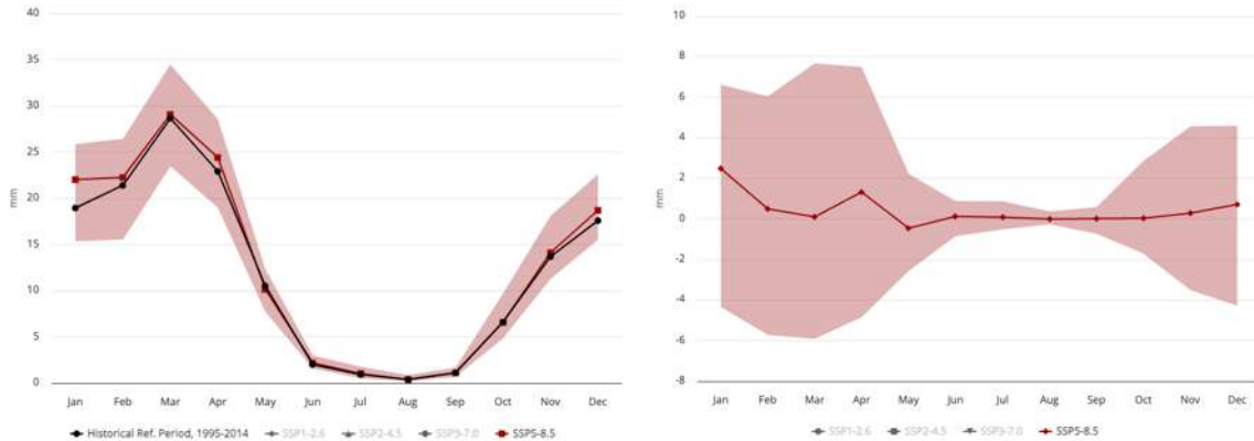
Figure 17-23 Projected Precipitation Climatology (Left) and Anomaly (Right) for 2020-2039 (Annual) for the Project Region; (Ref. Period: 1995-2014), SSP5-8.5, Multi-Model Ensemble
