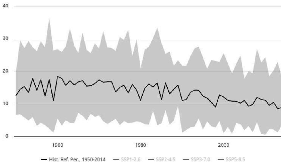
Figure 17-3 Historical Climatology of Number of Ice Days (Tmax < 0°C) in the Project Area for 1950-2014
