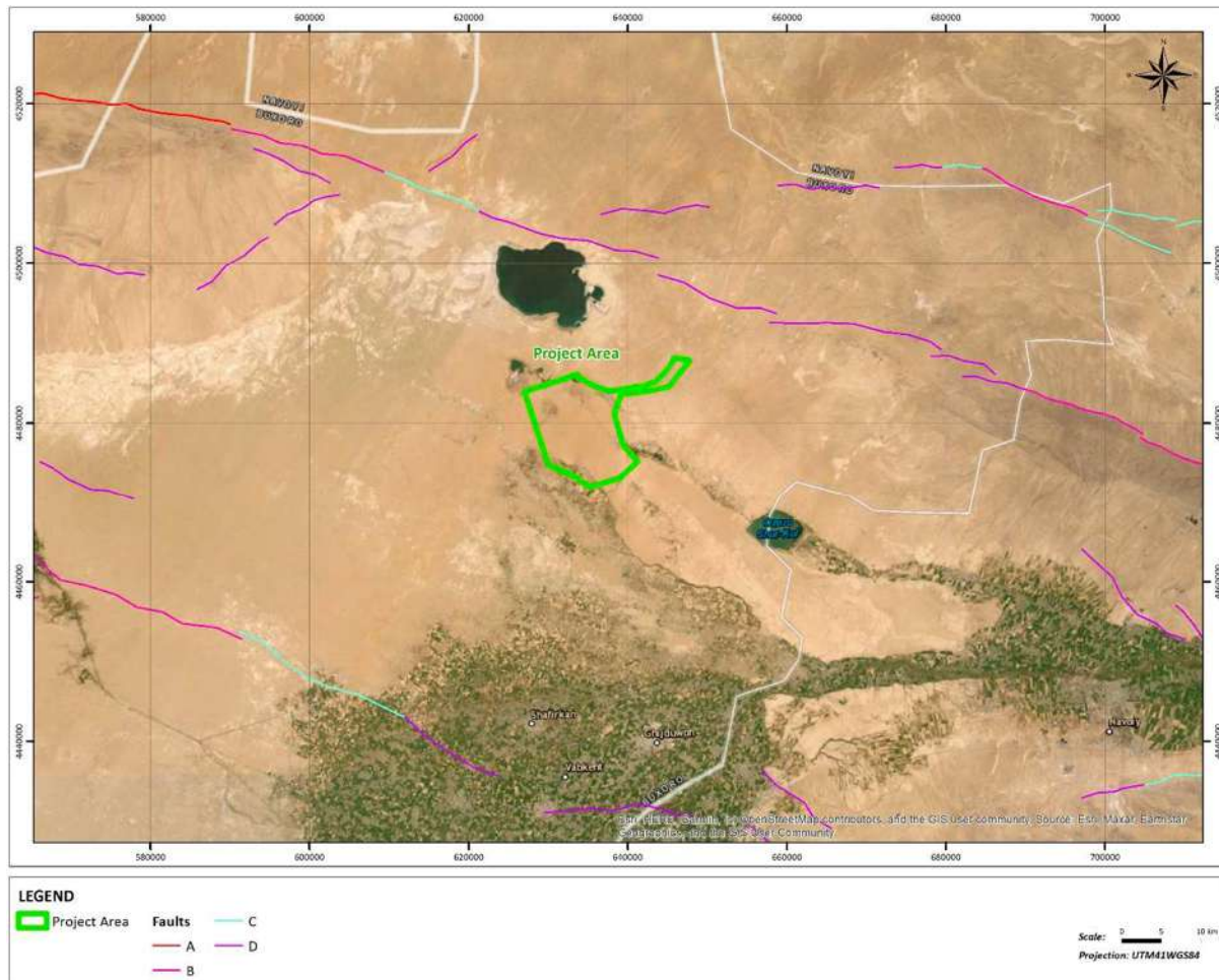
Figure 8-7 Active Fault Line Along the Project Site (UzAssystem, 2024a) 15
