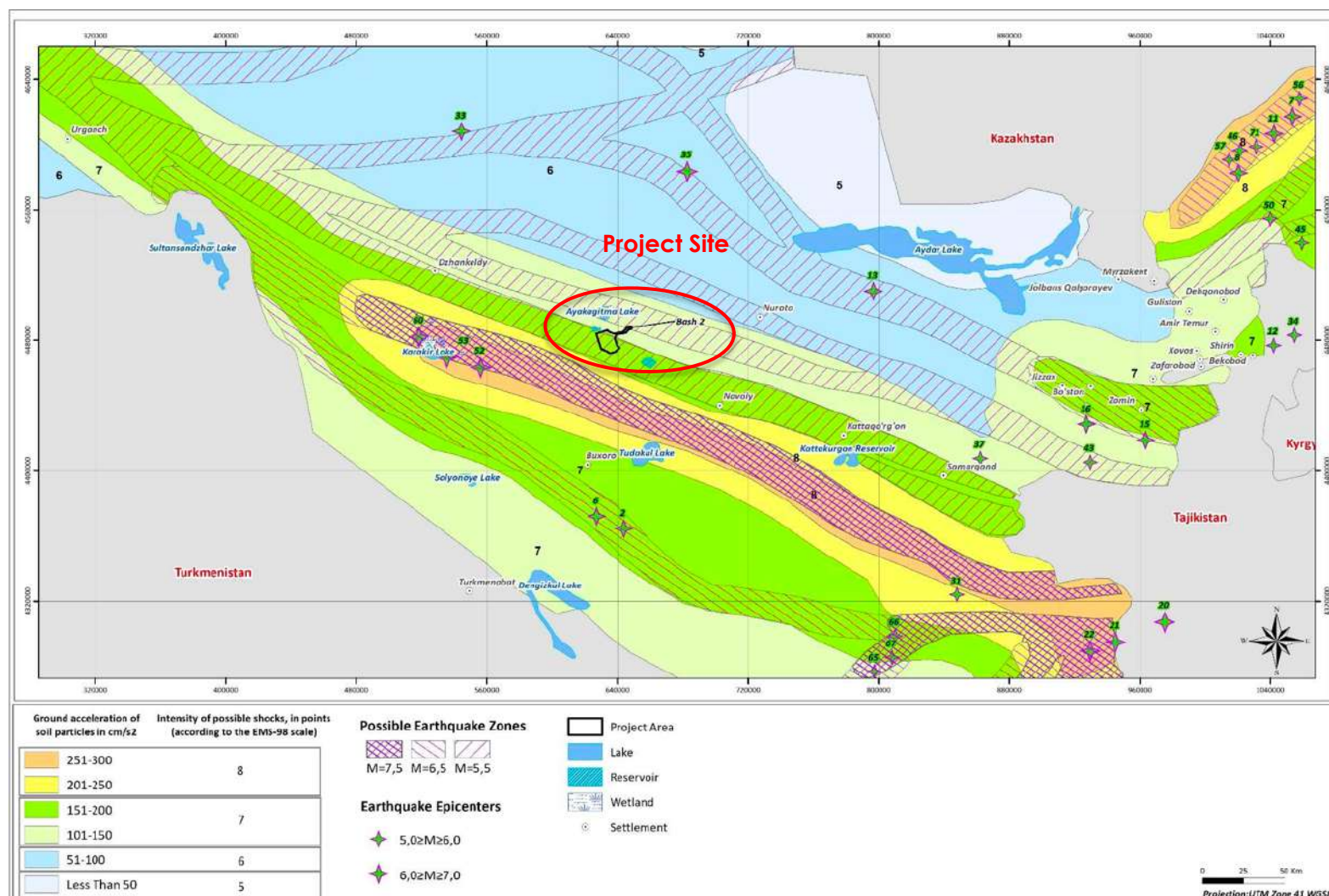
Figure 8-6 Location of Earthquakes with M > 5 in Relation to the Bash Project Site (UzAssystem, 2024a) 15
