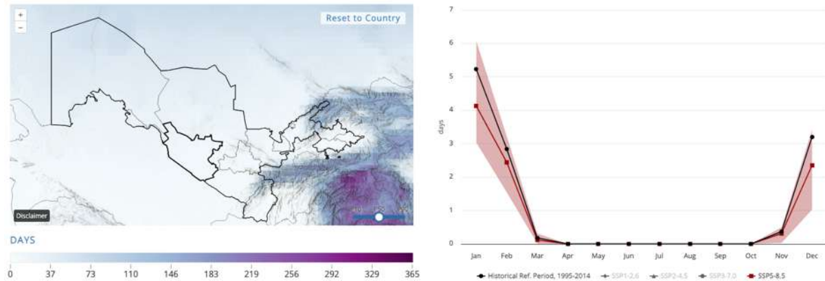
Figure 17-17 Projected Number of Ice Days ( T_{max} < 0^{\circ}\text{C} ) for the Project Area (2020-2039), SSP5-8.5, 50 th Percentile
