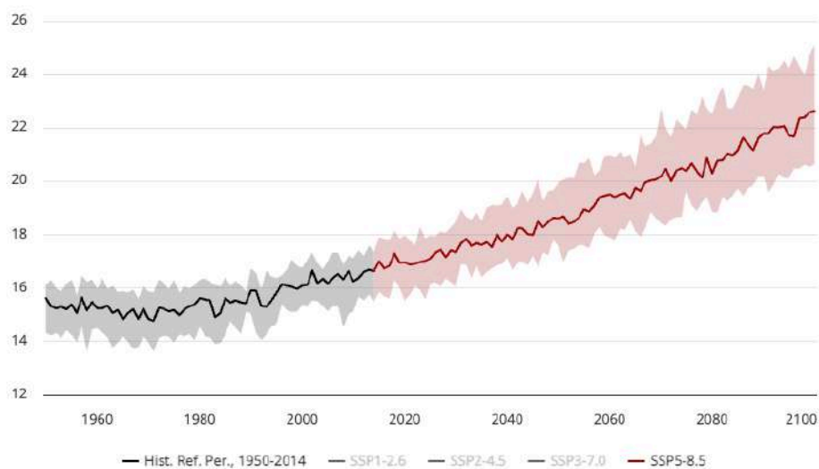
Figure 17-9 Projected Average Mean Surface Air Temperature for the Project Region; (Ref. Period: 1995-2014), SSP5-8.5, Multi-Model Ensemble
