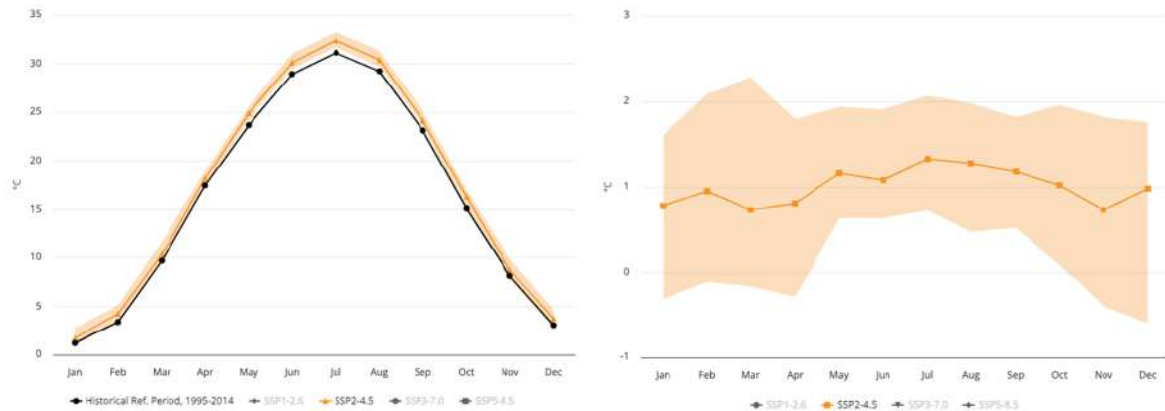
Figure 17-4 Projected Climatology (Left) and Anomaly (Right) of Average Mean Surface Air Temperature for 2020-2039 (Annual) for the Project Region; (Ref. Period: 1995-2014), SSP2-4.5, Multi-Model Ensemble
