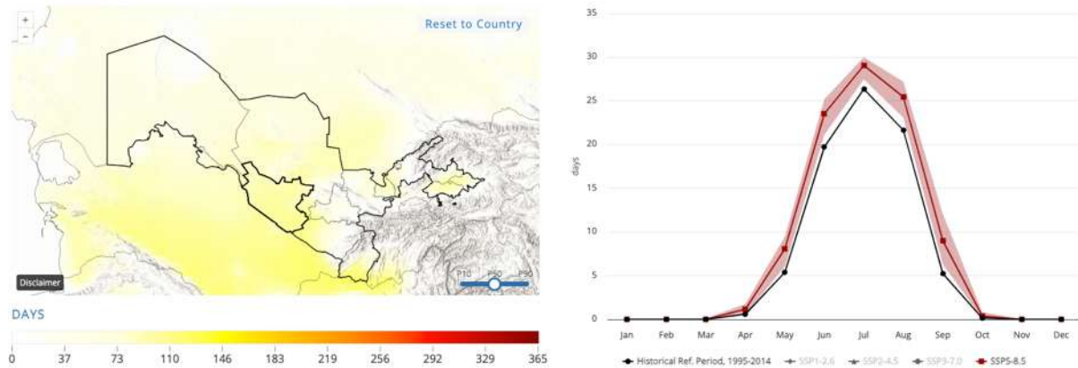
Figure 17-12 Projected Number of Hot Days ( T_{max} > 35^{\circ}\text{C} ) for the Project Area (2020-2039), SSP5-8.5, 50 th Percentile
