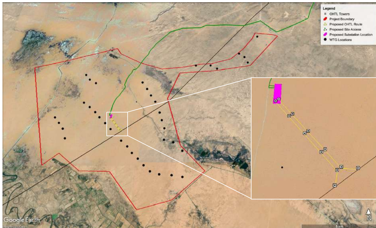
Figure 2-13 Project OHTL connecting to the existing Bash-Karakul OHTL Route
