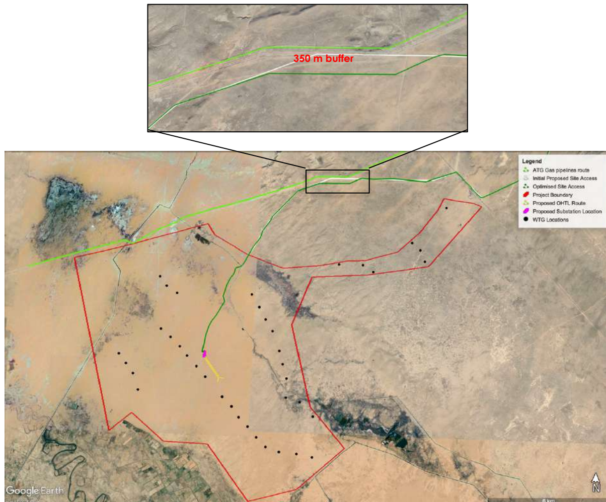
Figure 2-23 Optimised Site Access Road
