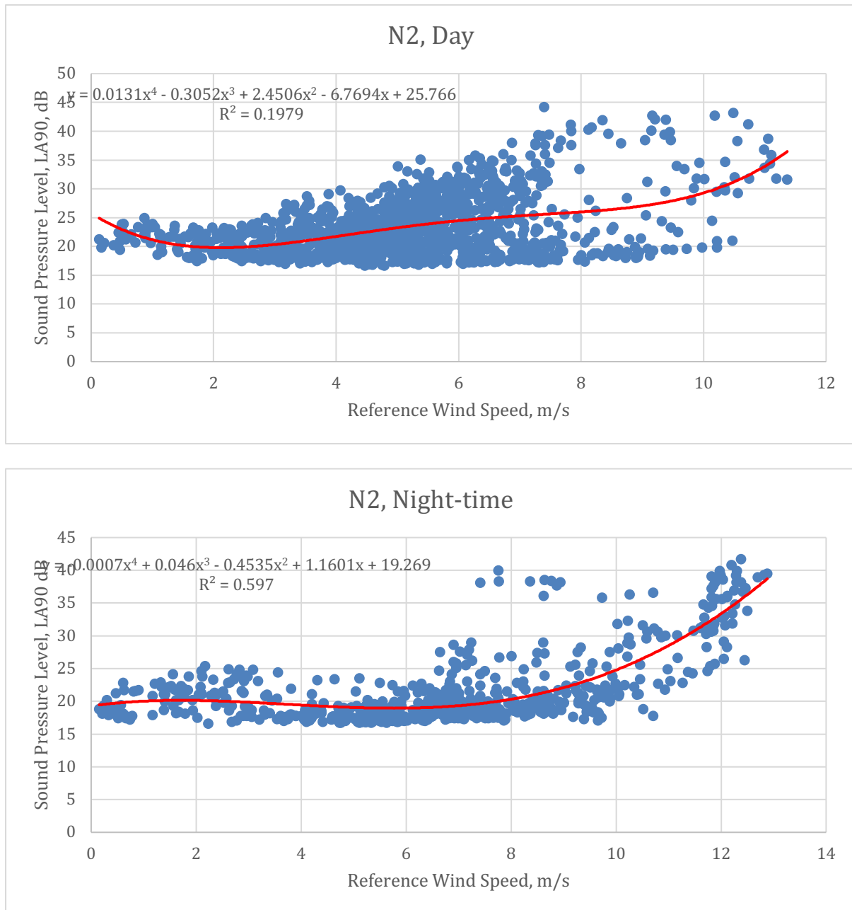
Figure 6-3 Regression Analysis at Survey Location N2
