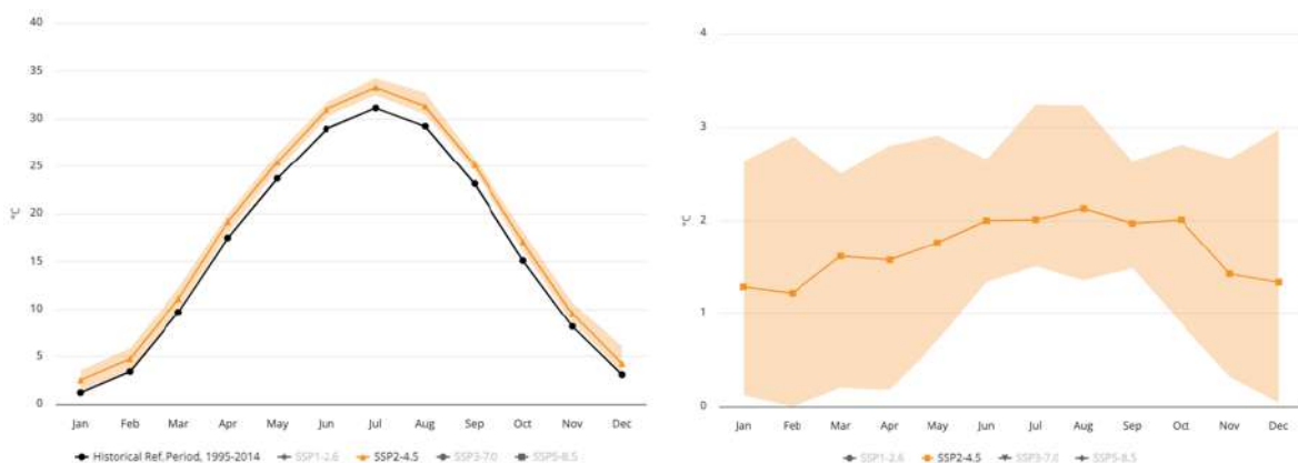
Figure 17-5 Projected Climatology (Left) and Anomaly (Right) of Average Mean Surface Air Temperature for 2040-2059 (Annual) for the Project Region; (Ref. Period: 1995-2014), SSP2-4.5, Multi-Model Ensemble
