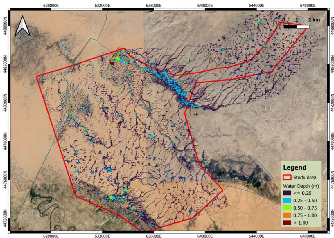
Figure 8-11 Water Depths due to 100-year Storm with DEM (UzAssystem, 2024c) 17
