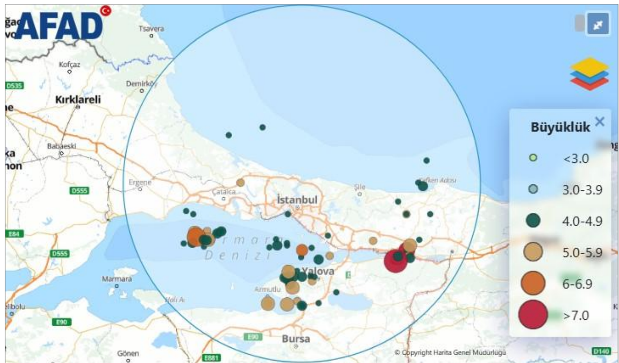
Figure 4-8 Magnitude of M \geq 4.5 Earthquakes within a 100 km radius of the Project Area
