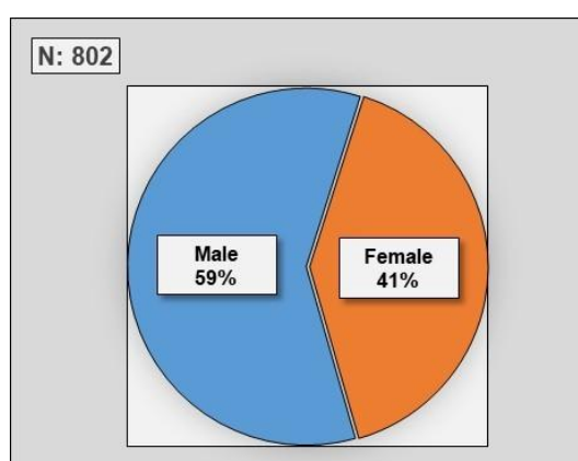
Figure 4-32 Gender distribution of the respondents, Household Survey, July 2025 (N:802)
