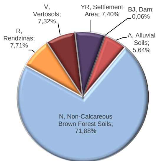
Figure 4-3 Major Soil Groups Data within the Project's Aol
