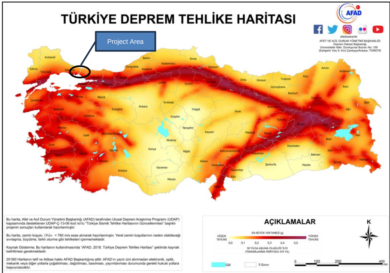
Figure 4-6 Earthquake Hazard Map of Türkiye with Project Area Marked
