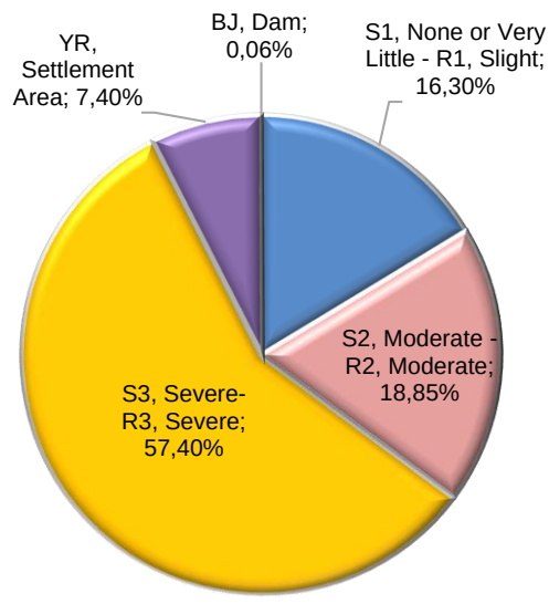
Figure 4-4 Erosion Levels Data within the Project's Aol
