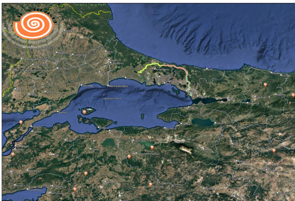
Figure 4-9 Geological Heritage Sites at and Around Project Route
