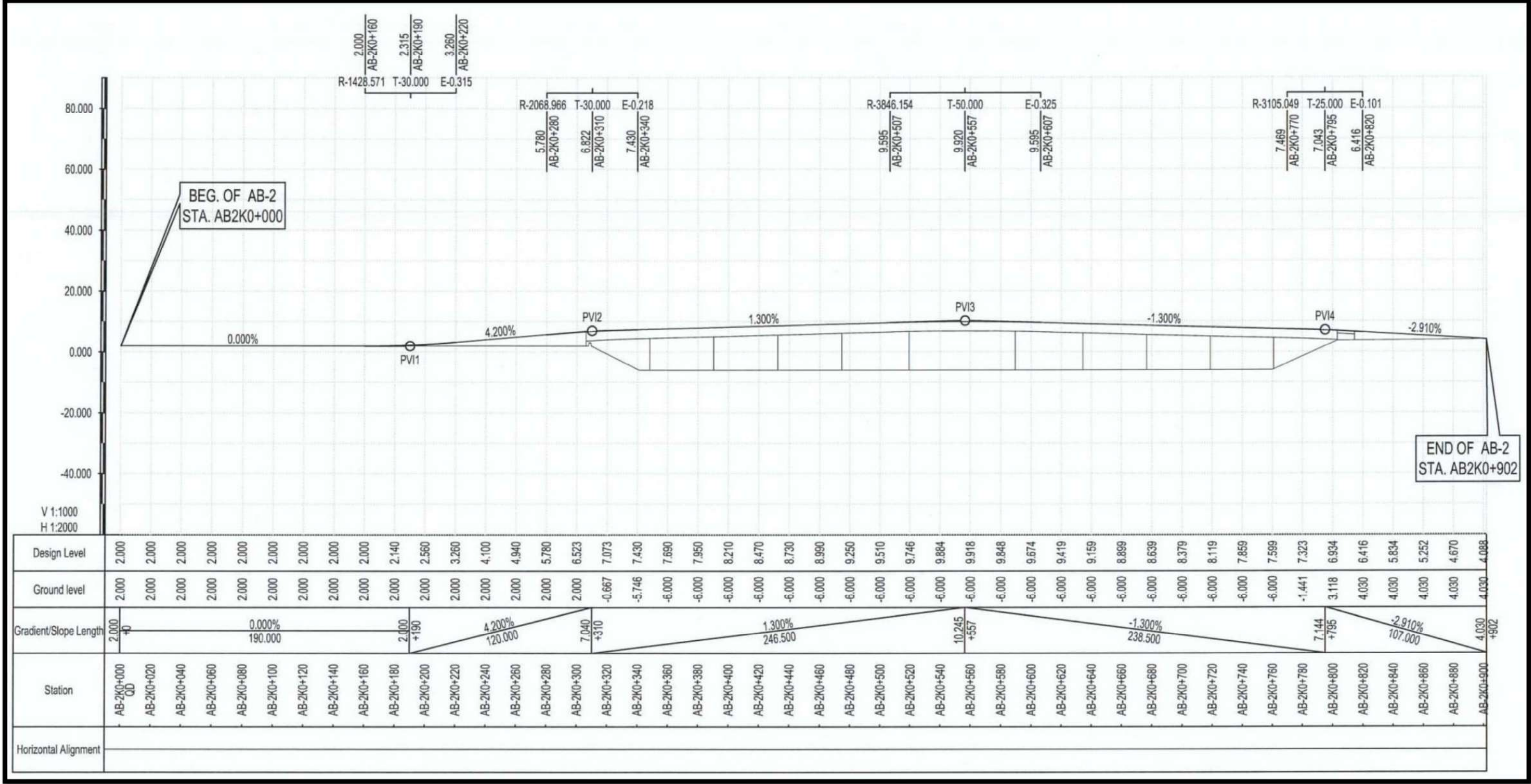
Figure 1.11 Road Profile of Vehicular and Pedestrian (Concrete) Bridge
