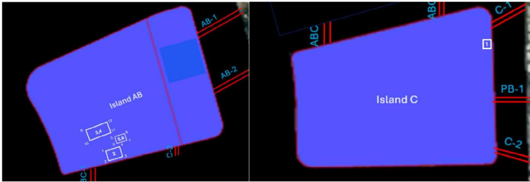
Figure 1.16 Location of the Temporary Support Facilities for the Construction of Inter-Island and Mainland-Connecting Bridge Structures
