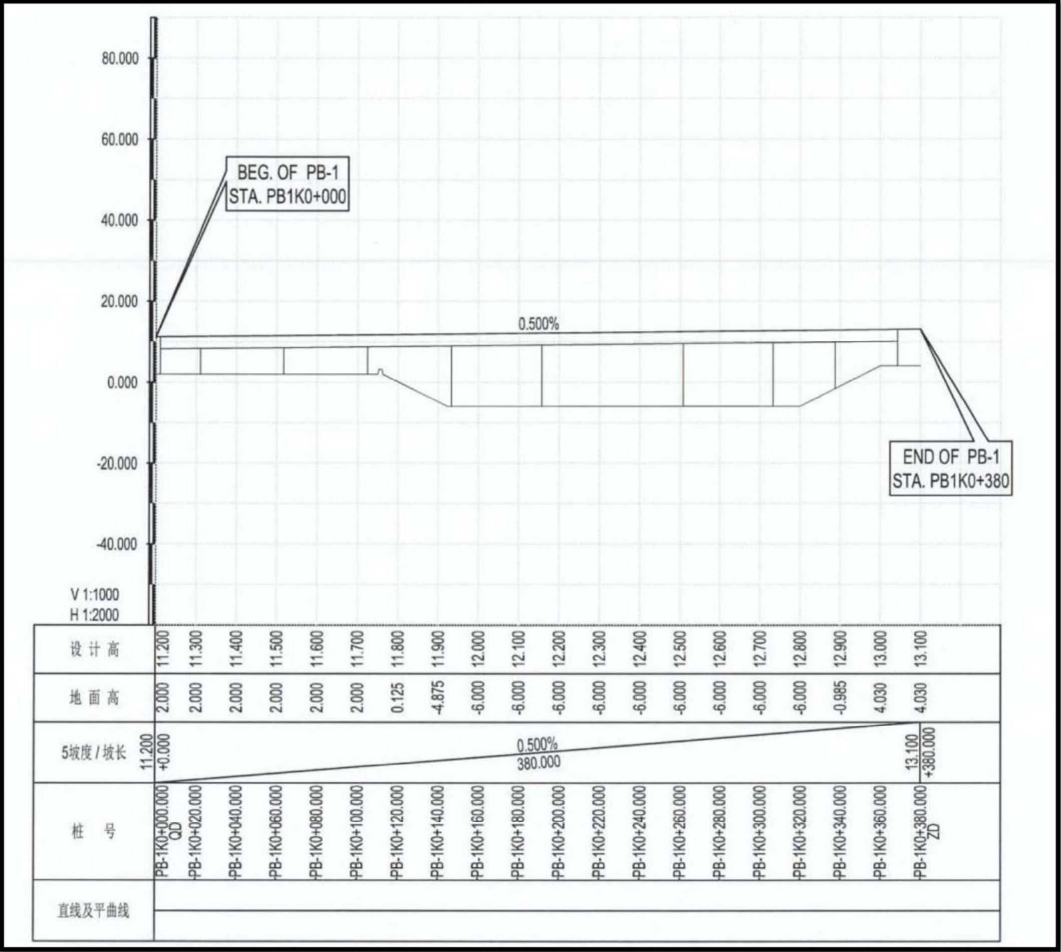
Figure 1.15 Road Profile of Pedestrian Bridge W
