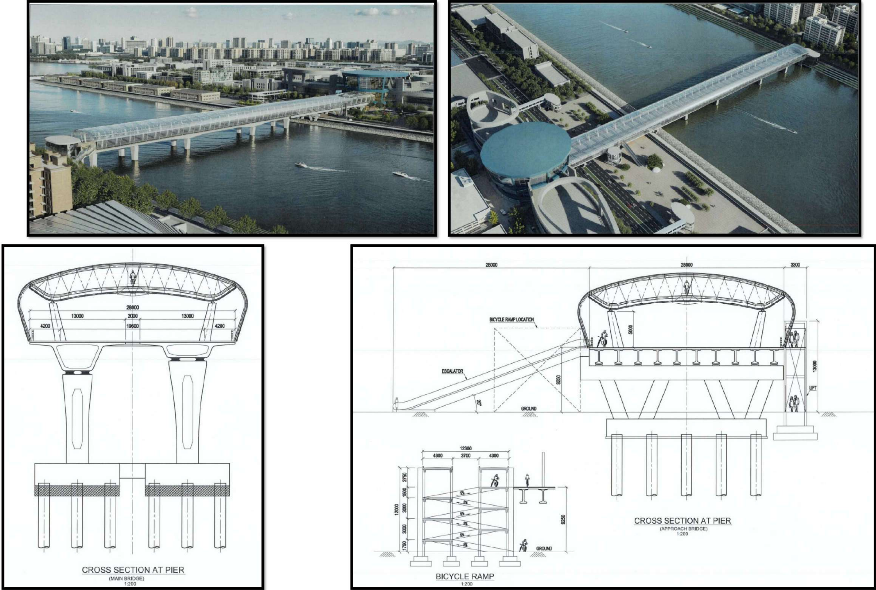
Figure 1.12 Perspective and Cross Section View of Pedestrian Bridge W
