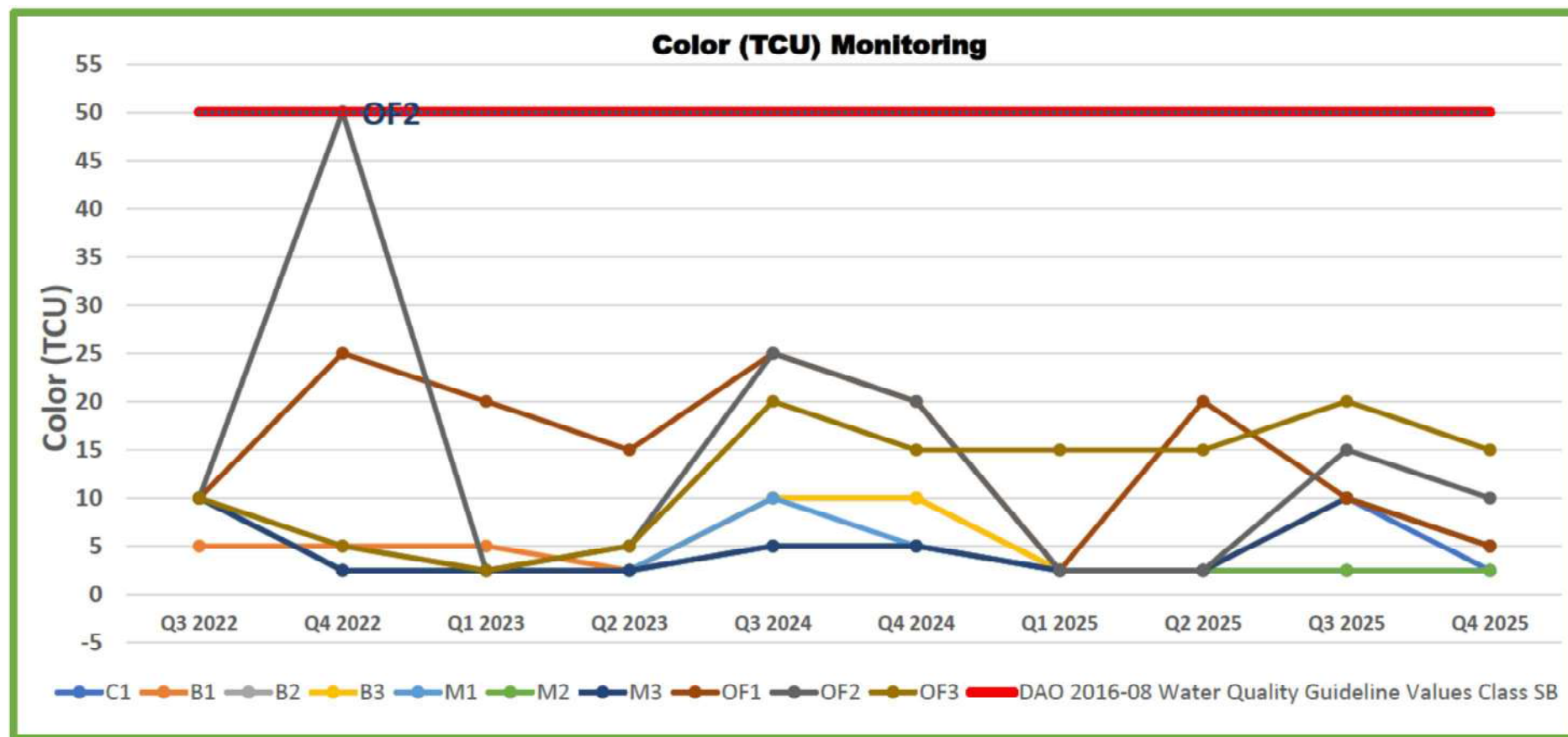
Figure 5.10 Color Monitoring
