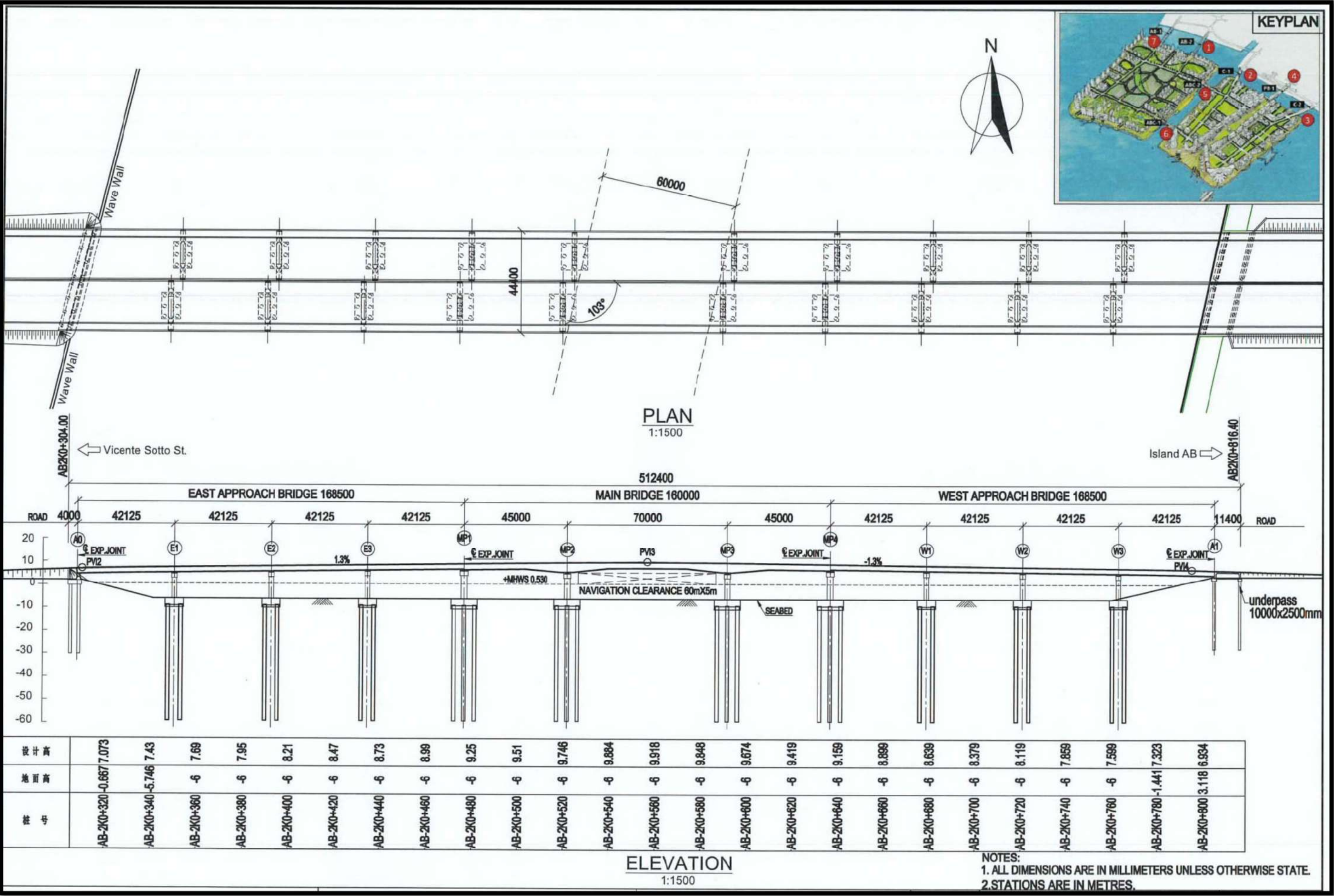
Figure 1.10 General Arrangement of Concrete Bridge
