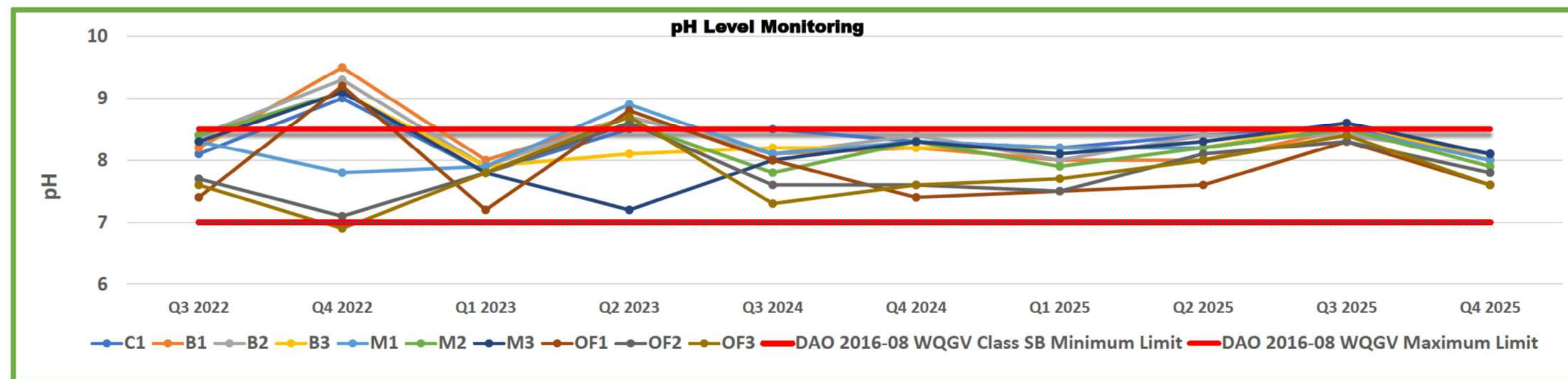
Figure 5.8 pH Monitoring
