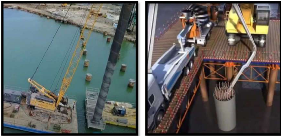
Figure 1.19 Offshore Pile Foundation Construction
