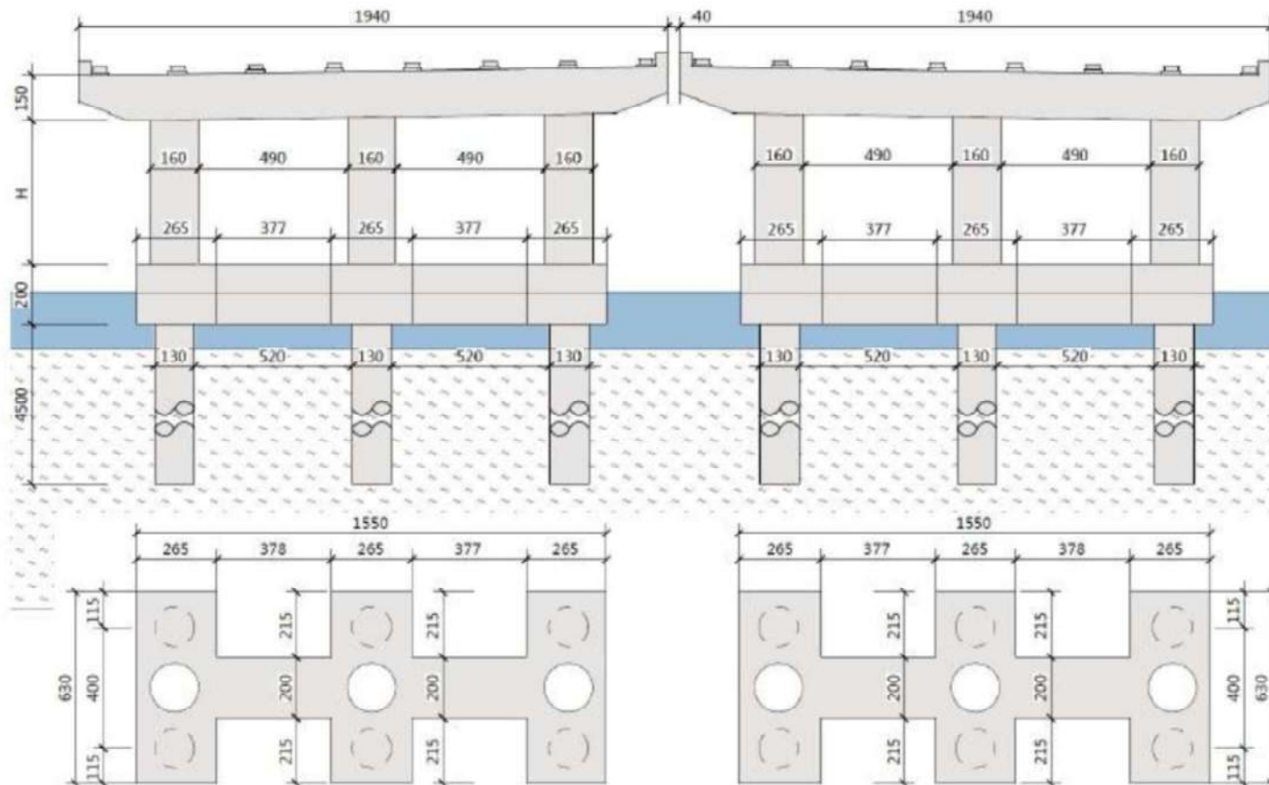
Figure 1.17 Initial Structural Concept for the Bridges - Substructure
