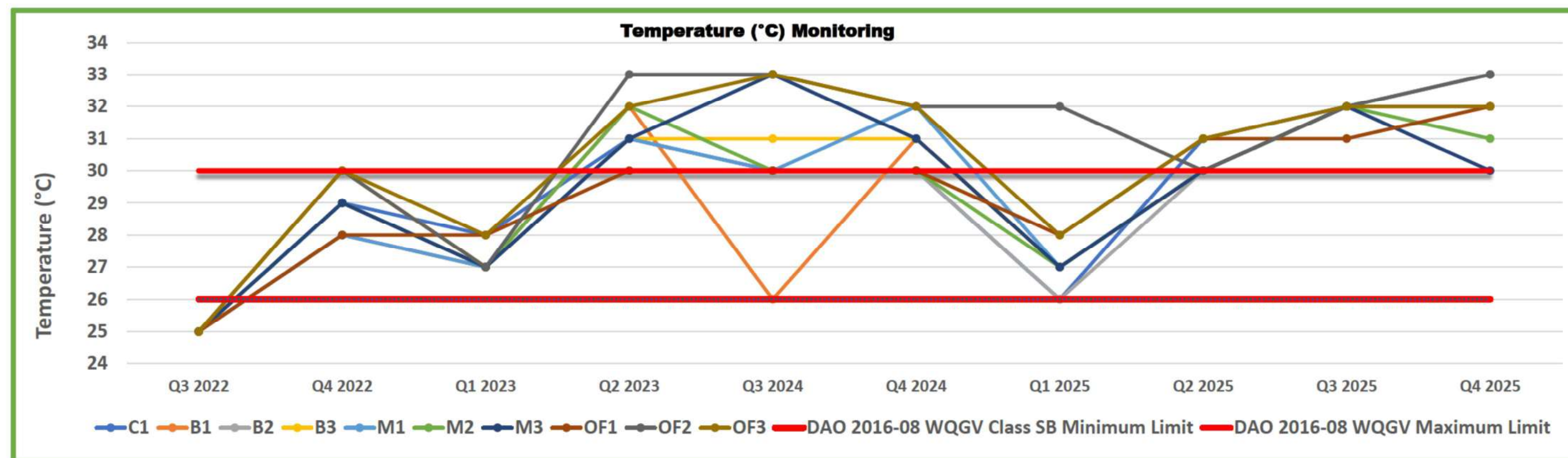
Figure 5.9 Temperature Monitoring
