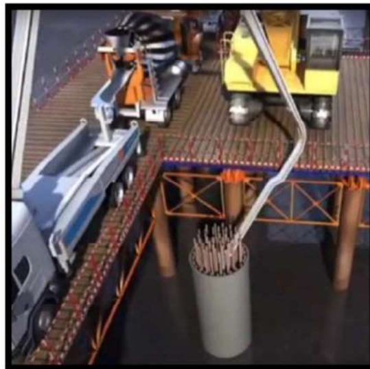
Figure 1.25 Offshore Pile Foundation Construction with Enclosure
