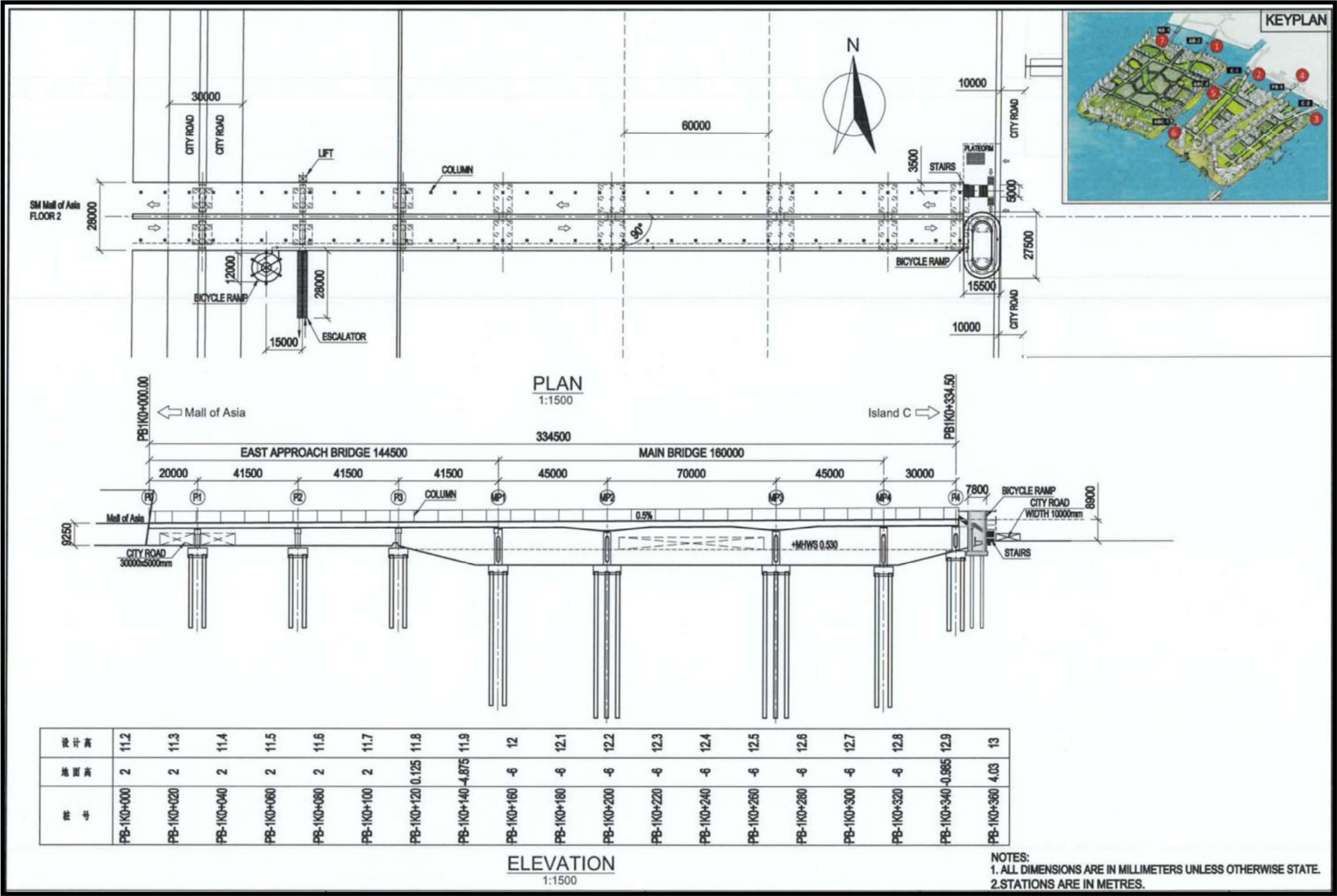
Figure 1.14 General Arrangement of Pedestrian Bridge W
