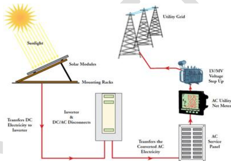
Figure 3-5 Typical Conventional Solar PV Power Plant Component 7
