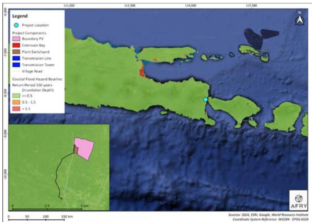
Figure 7-5 Baseline Coastal Flood Hazard
