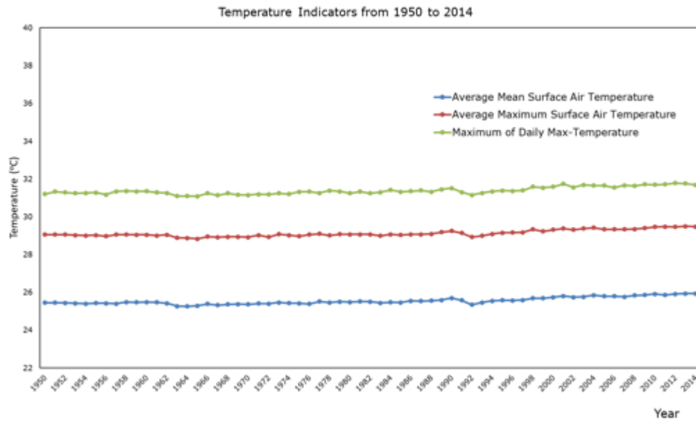
Figure 7-1 Historical Temperature Indicators
