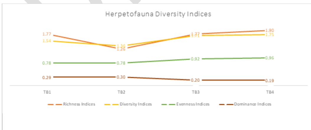
Figure 4-45 Diversity, evenness, and richness indices of herpetofauna species
