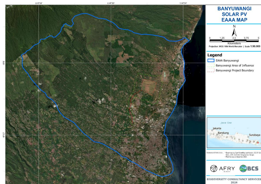
Figure 4-24 Ecologically Appropriate Area of Analysis of Banyuwangi Site
