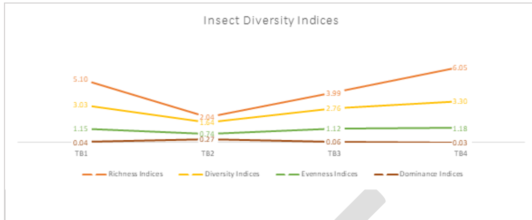
Figure 4-48 Diversity, evenness, and richness indices of herpetofauna species
