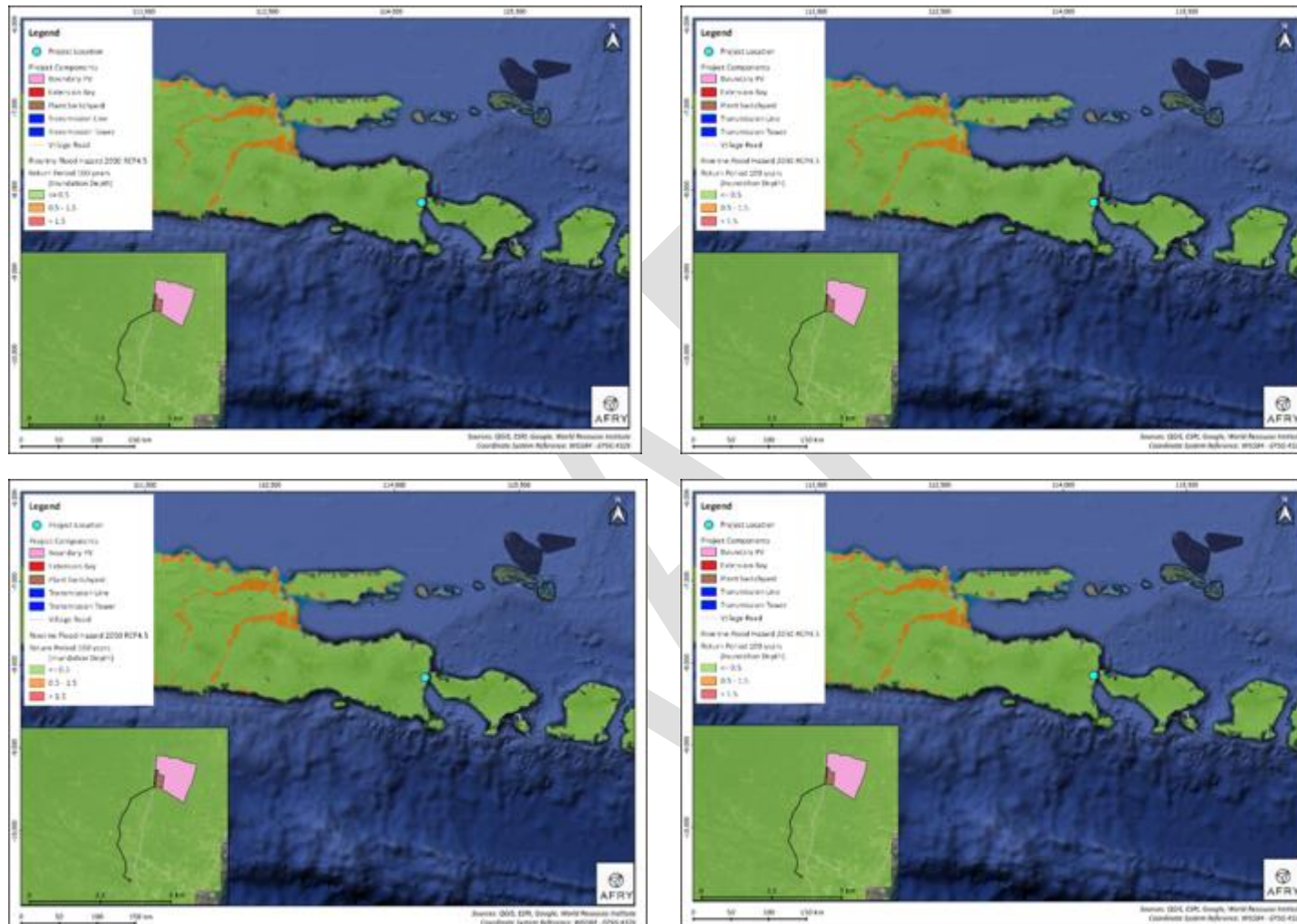
Figure 7-7 Projection of Riverine Flood Hazard in 2030 and 2050 under RCP 4.5 and RCP 8.5 Scenarios
