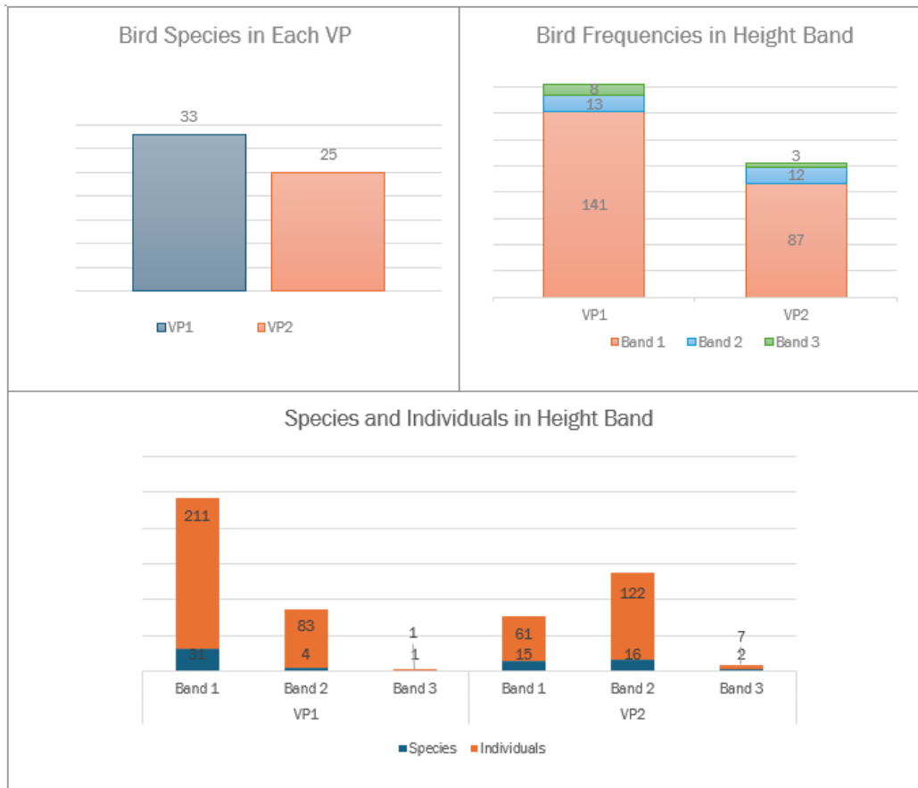
Figure 4-36 Species number, frequencies, and individuals in height band in each VP
