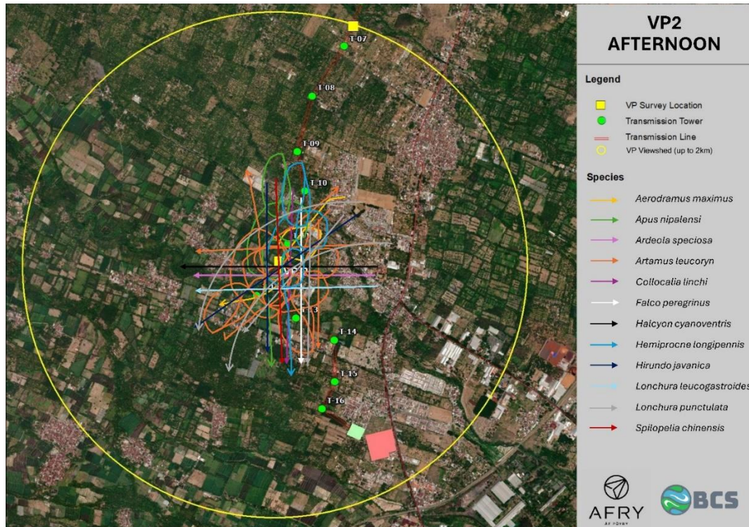
Figure 4-40 Birds Flight Direction Illustration within VP2 Location during Afternoon Observation
