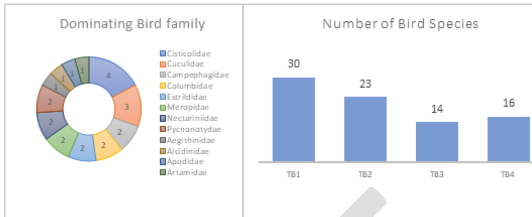
Figure 4-29 Dominating bird family and number of bird species in different transects
