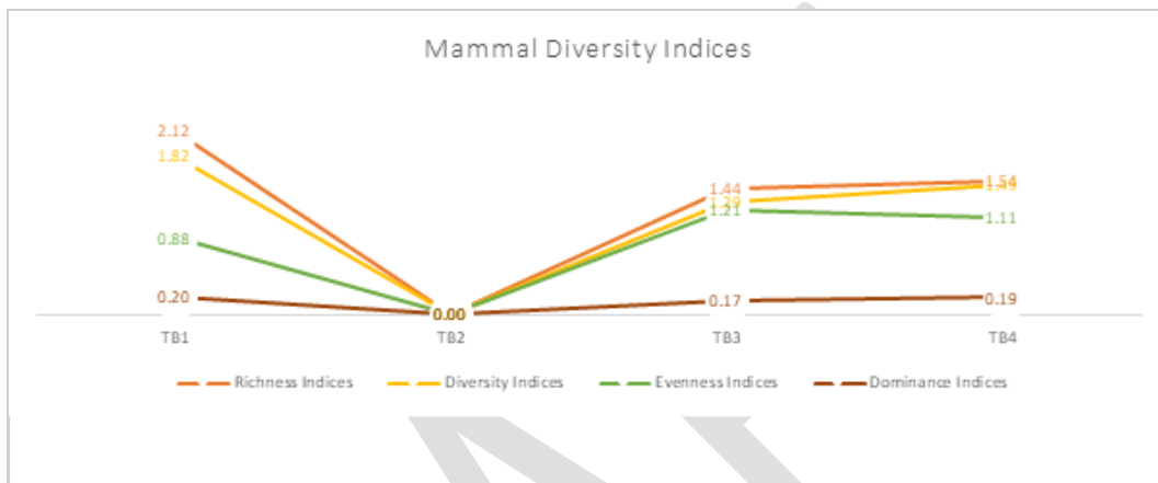
Figure 4-42 Diversity, evenness, and richness indices of mammal species
