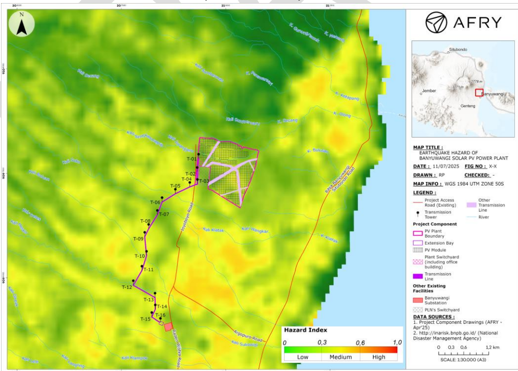
Figure 4-59 Earthquake hazard index of Banyuwangi Solar PV Power Plant
