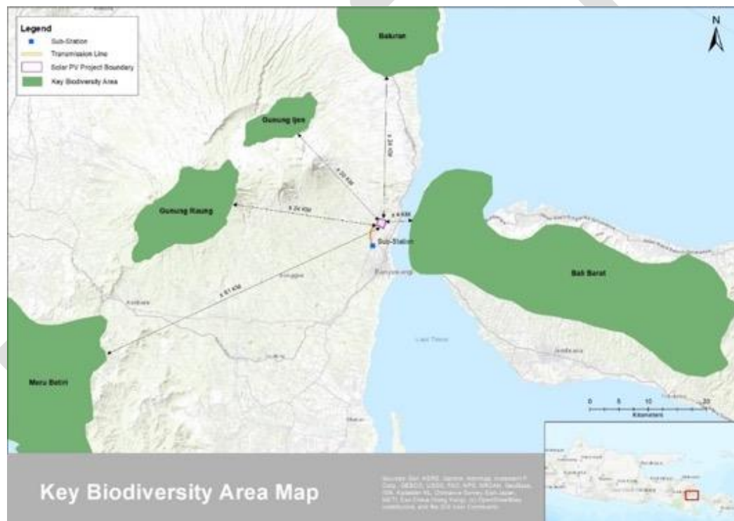
Figure 4-21 Key Biodiversity Area within 50km of Banyuwangi Site
