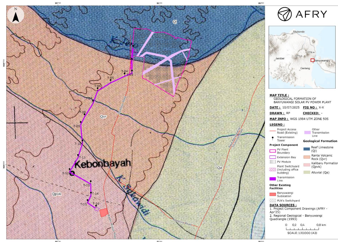
Figure 4-3 Geological Maps of Banyuwangi Quadrangle
