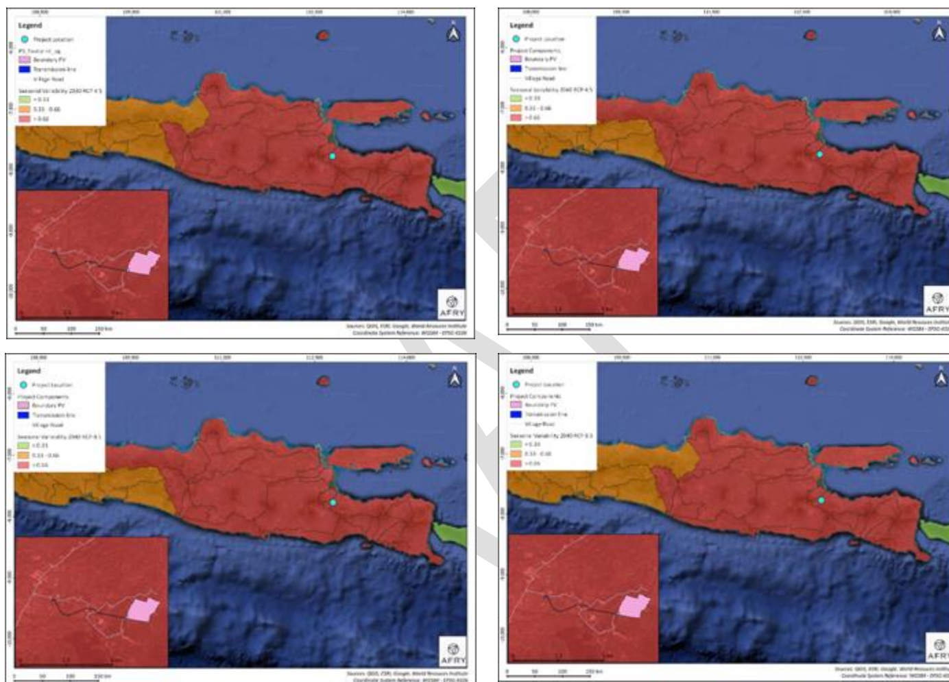
Figure 7-9 Projection of Seasonal Water Availability in 2030 and 2040 under RCP 4.5 and RCP 8.5 Scenarios
