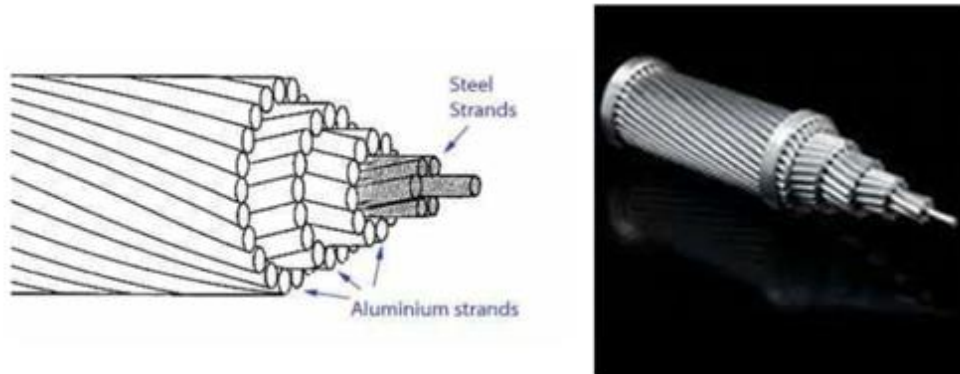
Figure 3-9 Cross-Sectional View of Typical ACSR OHL Conductor
