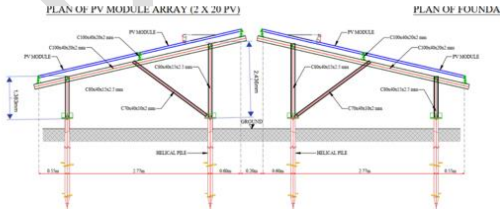
Figure 6-1 Typical Ground Mounted PV Foundation and Module Array
