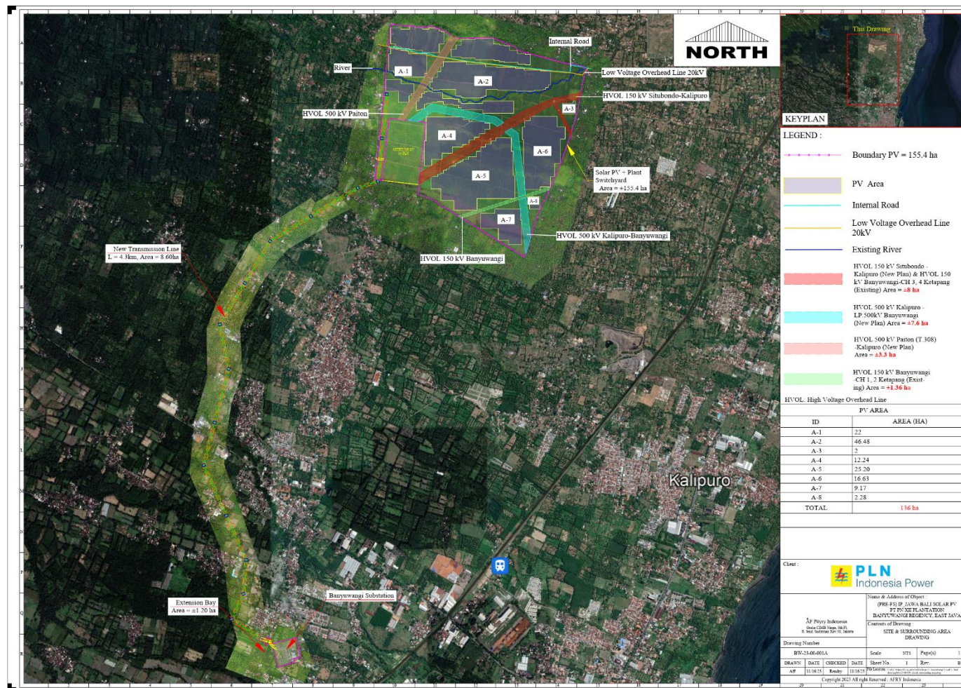
Source: Source: Feasibility Study Report for 100 MWac Java Land Based Solar PV Power Plants PLTS Banyuwangi, 2025 Figure 3-4 General plant layout and its facilities for Banyuwangi PV
