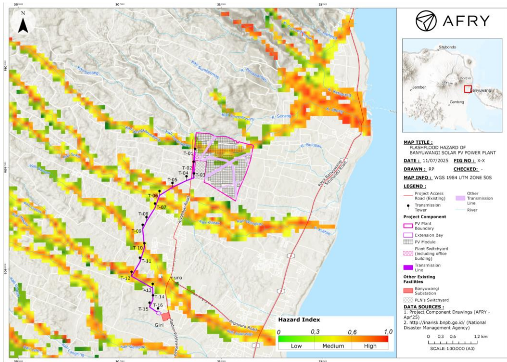
Figure 4-58 Flash flood hazard index of Banyuwangi Solar PV Power Plant
