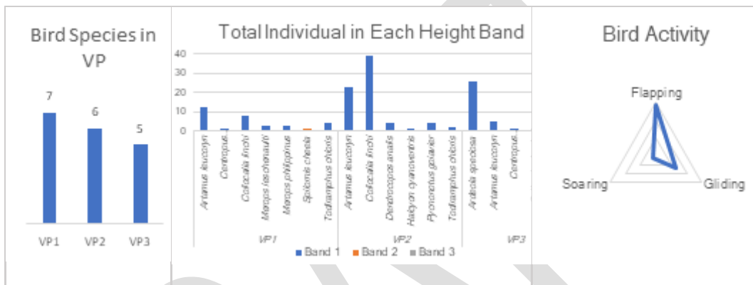
Figure 4-32 Bird Species in VP, Total Individual in Each Height Band and Bird Activity
