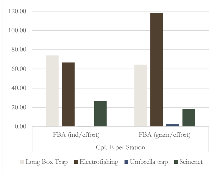
Figure 4-54 Catch per unit effort (individual and biomass comparison) of Ichthyofauna in Panawar River
