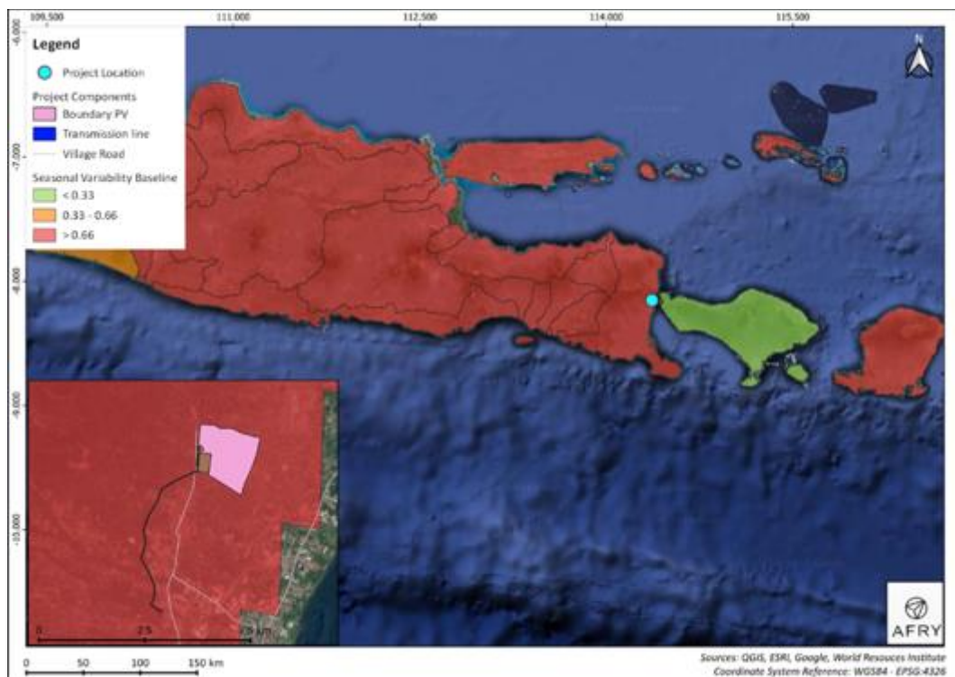
Figure 7-3 Baseline Seasonal Variability
