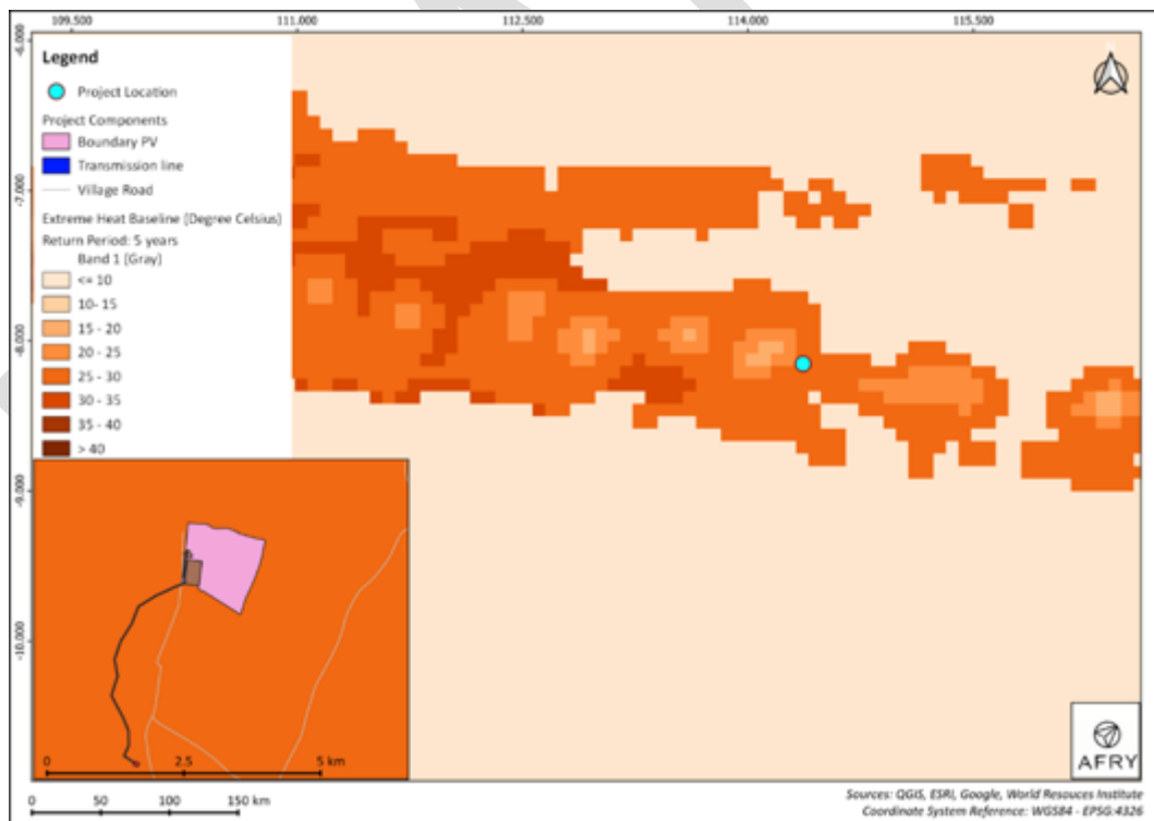
Figure 7-2 Baseline Extreme Heat Hazard in the Project Area
