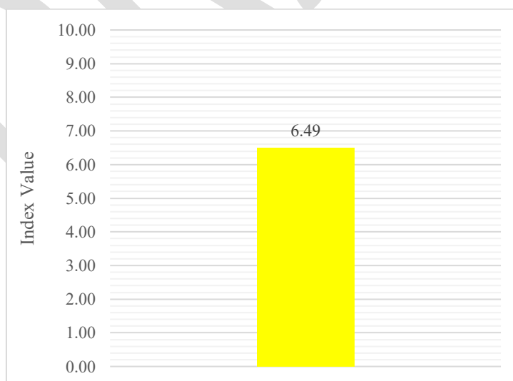
Figure 4-56 Family Biotic Index in FBA
