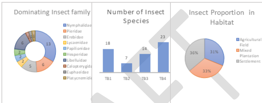
Figure 4-47 Number of insect families and species in different transects and habitats
