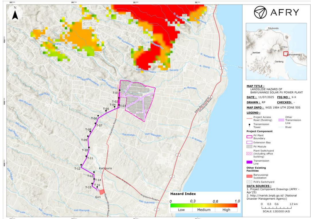
Figure 4-57 Landslide hazard index of Banyuwangi Solar PV Power Plant
