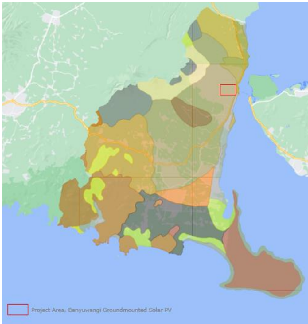
Figure 4-4 Soil Type of Banyuwangi Regency
