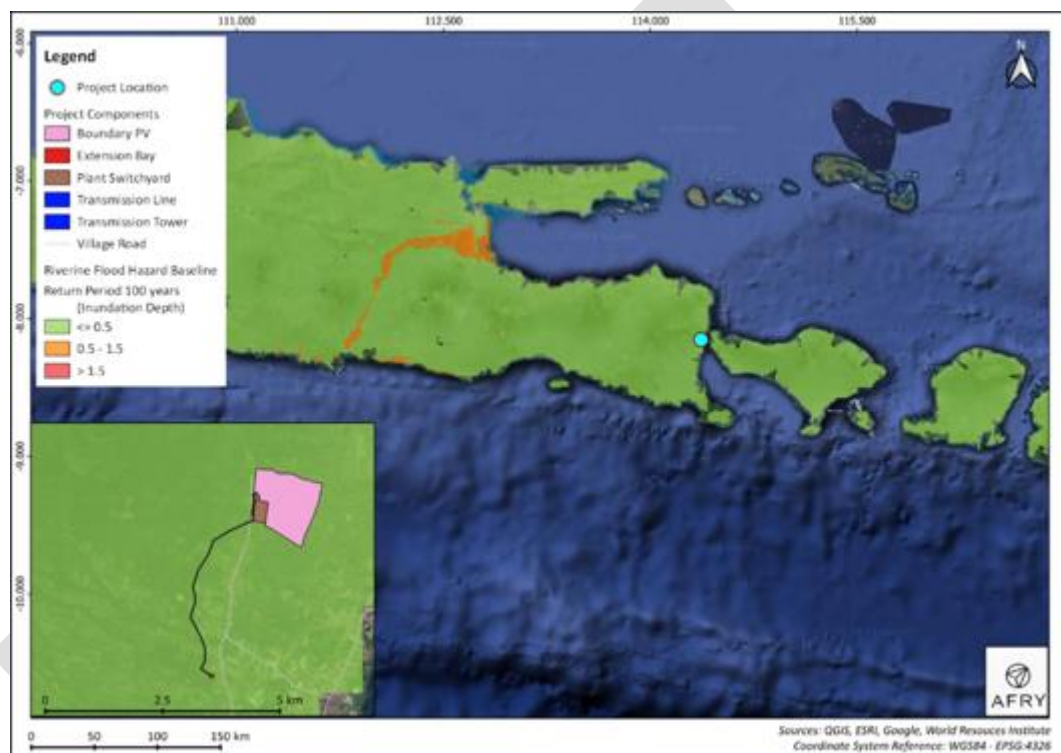
Figure 7-4 Baseline Riverine Flood Hazard
