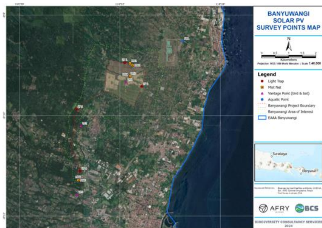
Figure 4-26 Terrestrial and Aquatic Biodiversity Survey Locations of Banyuwangi Ground Mounted Solar PV
