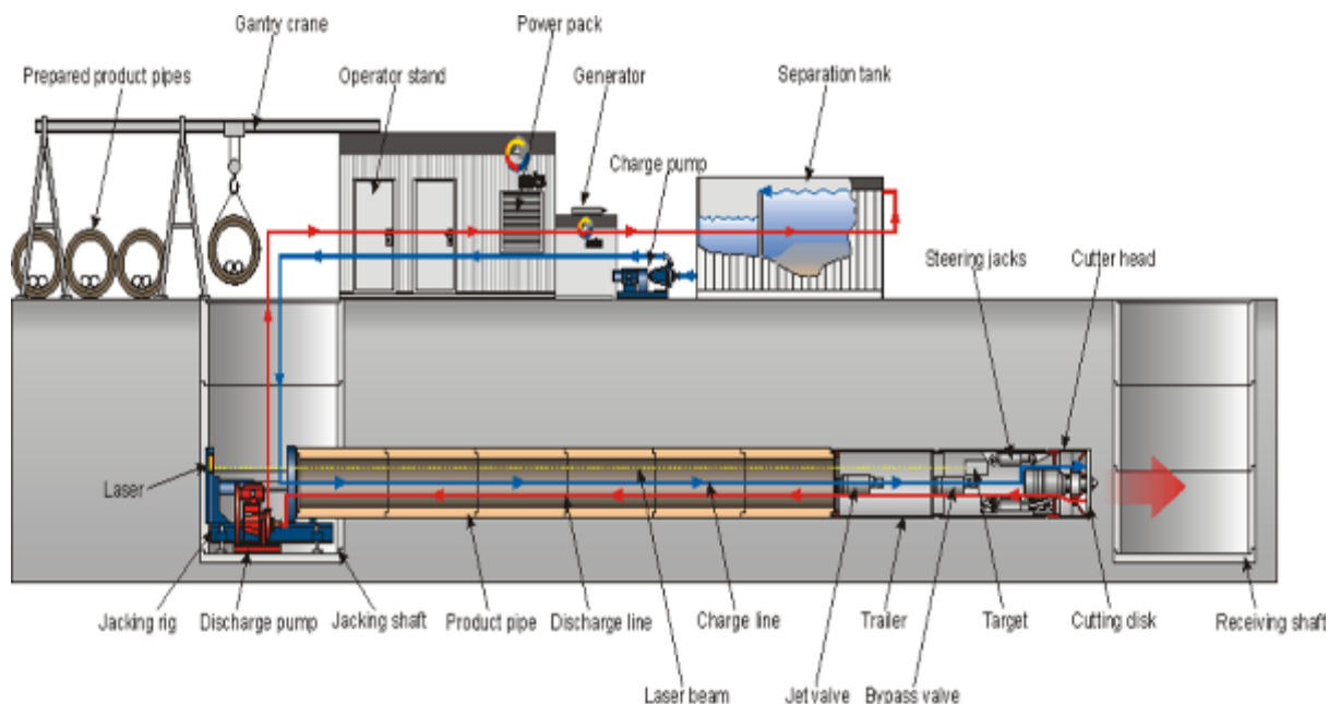
Figure 3-4: Micro-Tunneling Schematic
