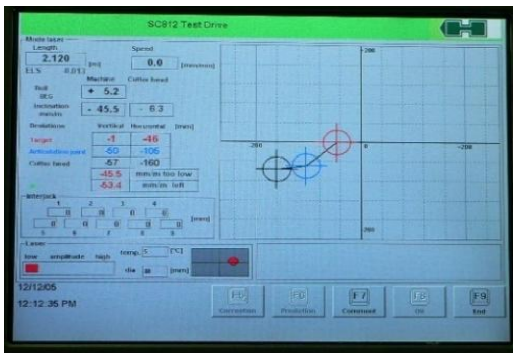
Figure 3-7: Typical Control Unit Screens
