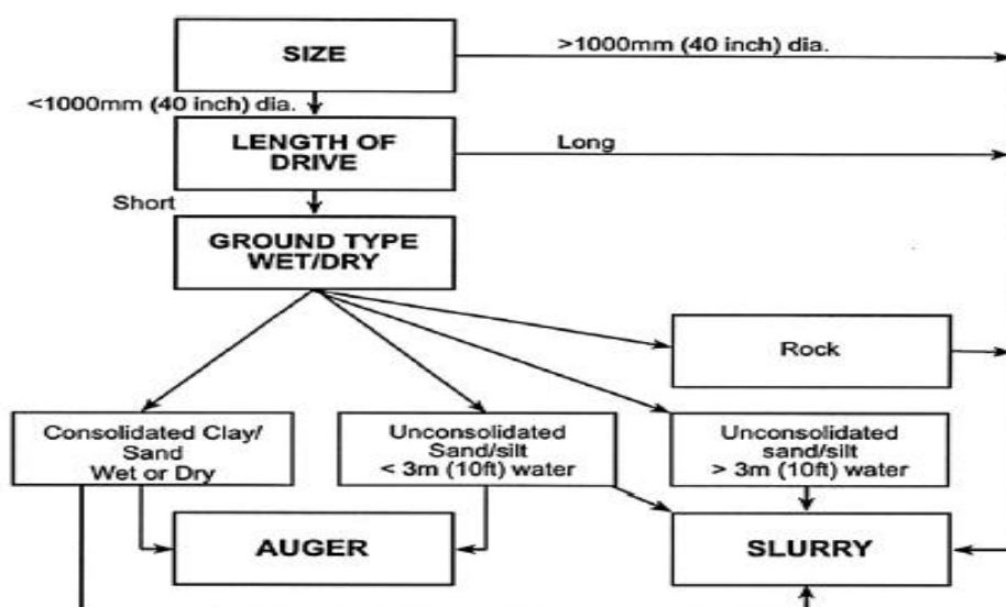
Figure 3-5: Determination of Tunneling Technique (from ASCE/CI 36-15)
