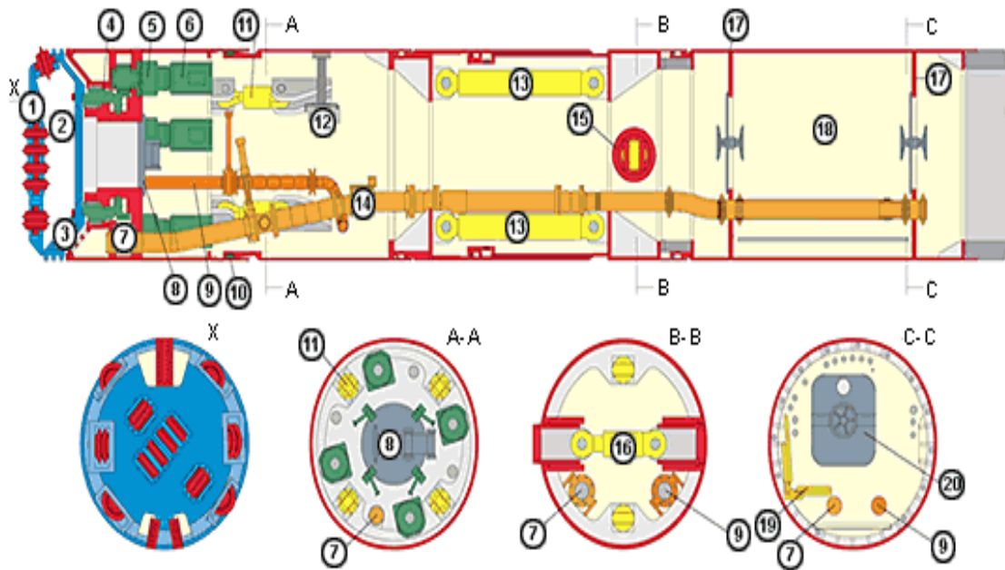
Figure 3-6: MTBM Component
