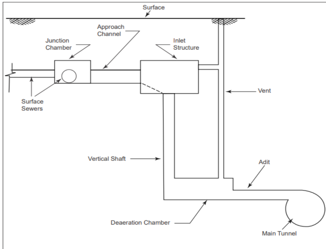
Figure 3-10: Drop Structure Design
